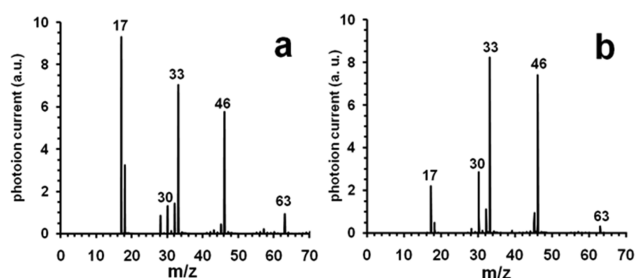
Figure 1. Typical mass spectra at 12.6 eV photoionization energy and a target temperature of 300 °C for (a) the thermal decomposition of HAN on a copper target, and (b) the catalytic decomposition of HAN on an iridium target.
