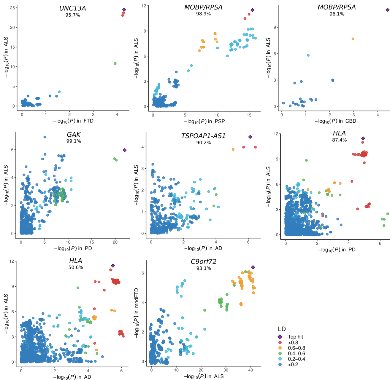
Extended Data Fig. 6 | Colocalization signals. Loci were selected for colocalization analysis when the top associated SNP was associated with any neurodegenerative disease at 5 \times 10^{-5} . For ALS, the European ancestries meta-analysis was used. Bayesian posterior probabilities for a shared variant driving risk of both traits (PP H4 ) are reported below locus names. Colors reflect LD between the variant and top associated SNP.
