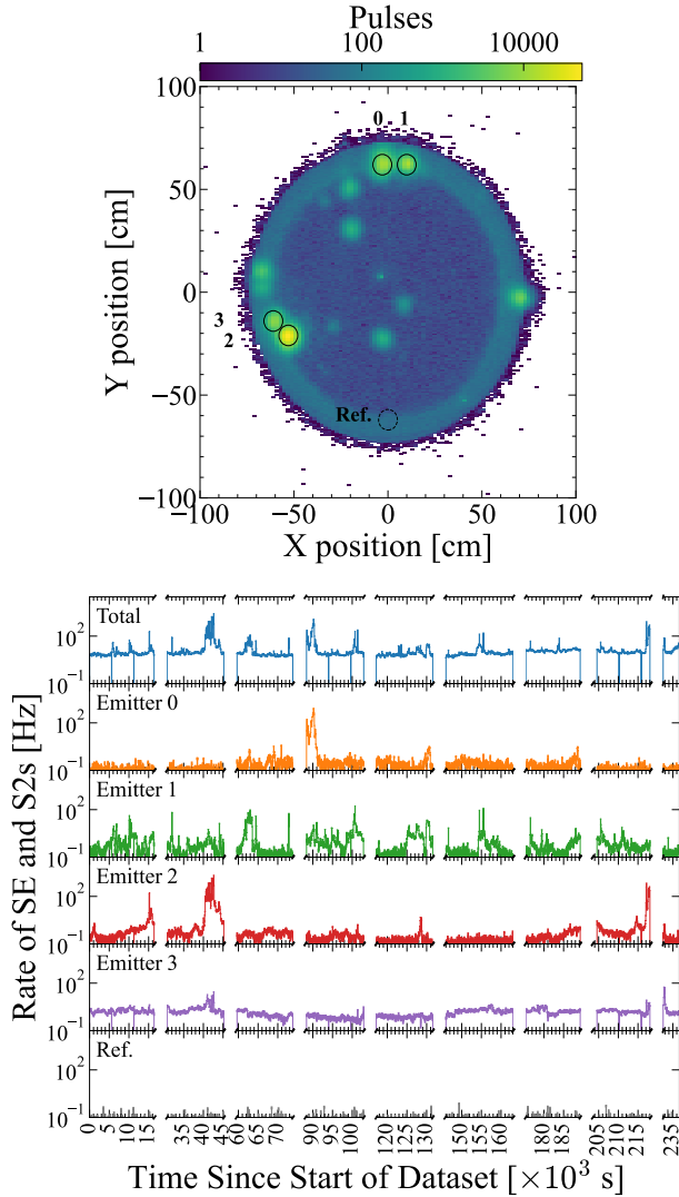
Figure 6: Reconstructed X-Y position distribution of S2 pulses (including SEs) in a randomly-triggered extraction region-only dataset (top). The ring feature is due to shadowing effects at the circumference of the TPC that cause S2 positions to be reconstructed inwards. Several X-Y locations, corresponding to active emitters as well as a lower rate reference region, are denoted with black circles and enumerated, and the rates of S2s in those localized regions are shown as a function of time in the bottom panel. Periods with a mixed trigger logic (i.e. not purely random-triggered) are excluded.
