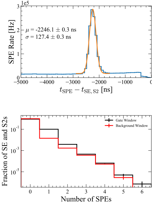
Figure 7: Rate of single photo-electrons (SPEs) preceding post-cuts S2 pulses (including SEs), shown in the top panel. The peak position ( \mu = -2246.1 \pm 0.3 ns) is consistent with the drift time associated with the LZ gate grid. The number of SPEs in a time window of \pm 5\sigma around the gate drift time (black) and within an equally-sized time window offset from the gate drift time (red) is shown in the bottom panel.
