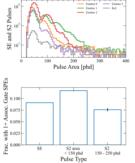
Figure 8: S2 pulse area spectra from both identified emitters and a reference region enumerated in Fig. 6, shown in the top panel. The bottom panel depicts the fraction of S2s of different pulse sizes with at least one correlated SPE, after subtracting the background from the uncorrelated SPE rate.
