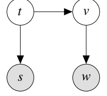
Figure 4: The probabilistic model used to predict the semantic properties of a word given its syntactic properties and surface form. Shaded circles are observed variables and empty circles are latent. See main text for details.
