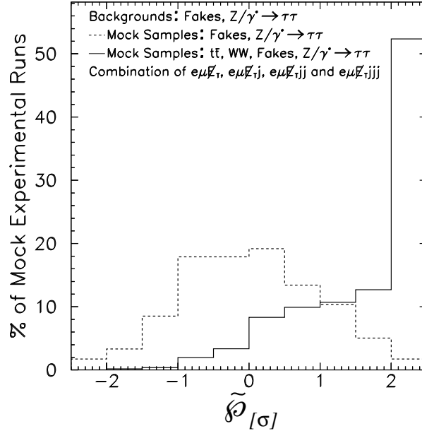
Figure 4.6: Distribution of \tilde{\mathcal{P}}_{[\sigma]} from combining the four exclusive final states e\mu\cancel{E}_T , e\mu\cancel{E}_T j , e\mu\cancel{E}_T jj , and e\mu\cancel{E}_T jjj . The background includes only Z/\gamma^* \rightarrow \tau\tau and fakes. The mock samples making up the distribution shown as the solid line contain WW and t\bar{t} in addition to Z/\gamma^* \rightarrow \tau\tau and fakes, and correspond to Fig. 4.5; the mock samples making up the distribution shown as the dashed line contain only Z/\gamma^* \rightarrow \tau\tau and fakes, and correspond to Fig. 4.4. All samples with \tilde{\mathcal{P}}_{[\sigma]} > 2.0 appear in the rightmost bin. The fact that \tilde{\mathcal{P}}_{[\sigma]} > 2.0 in 50% of the mock samples can be taken as a measure of Sleuth’s sensitivity to finding WW and t\bar{t} if we had no knowledge of the existence of the top quark or the possibility of W boson pair production.
