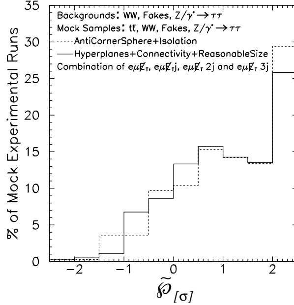
Figure 5.3: Distribution of \tilde{\mathcal{P}}_{[\sigma]} in an ensemble of mock experimental runs on the four exclusive final states e\mu\tilde{\mathcal{P}}_T , e\mu\tilde{\mathcal{P}}_{Tj} , e\mu\tilde{\mathcal{P}}_{T2j} , and e\mu\tilde{\mathcal{P}}_{T3j} . The background includes Z/\gamma^* \rightarrow \tau\tau , fakes, and WW . The mock samples making up the distributions contain t\bar{t} in addition to Z/\gamma^* \rightarrow \tau\tau , fakes, and WW .
