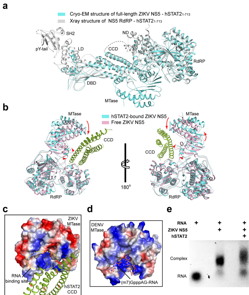
Extended Data Figure 6. Structural analysis of the ZIKV NS5-hSTAT2 interaction. a , Superposition of the crystal structure of NS5 RdRP-hSTAT2 1-713 (grey) and the cryo-EM structure of full-length NS5-hSTAT2 1-713 (cyan). While the cryo-EM structure contains the MTase domain, there is no change in the relative orientations of different domains between the two structures. b , Structural superposition of free (PDB 5TMH) and hSTAT2-bound ZIKV NS5. The conformational transition of the MTase domain of ZIKV NS5 from free state to the hSTAT2-bound state is indicated by arrows. For clarity, all the hSTAT2 domains, except for the CCD, were removed. c , Surface view of the MTase domain of ZIKV NS5 bound to hSTAT2 CCD (green ribbon). The four helices of the CCD are sequentially numbered from '1' to '4'. The potential RNA binding site is indicated by dashed circle. d , Surface of the DENV-3 MTase bound to viral cap-0 RNA (PDB 5DTO). e , hSTAT2 inhibition of ZIKV NS5-RNA binding assayed by electrophoretic mobility shift. Addition of NS5 to a cap-1 (m 7 GpppG 2' OMe) yeast mRNA (YLR164W, 749 nt) resulted in a shift of the
