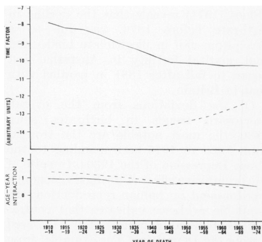
FIG. 4.—Variation in the time factors and age-year interaction terms. — Australia; - - - England and Wales.
