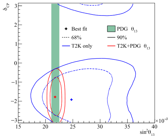
Fig. 23 68% and 90% credible intervals from the marginalized \sin^2 \theta_{13} - \delta_{CP} posterior distribution with (red) and without (blue) the reactor constraint (green band) applied, marginalized over both mass orderings
