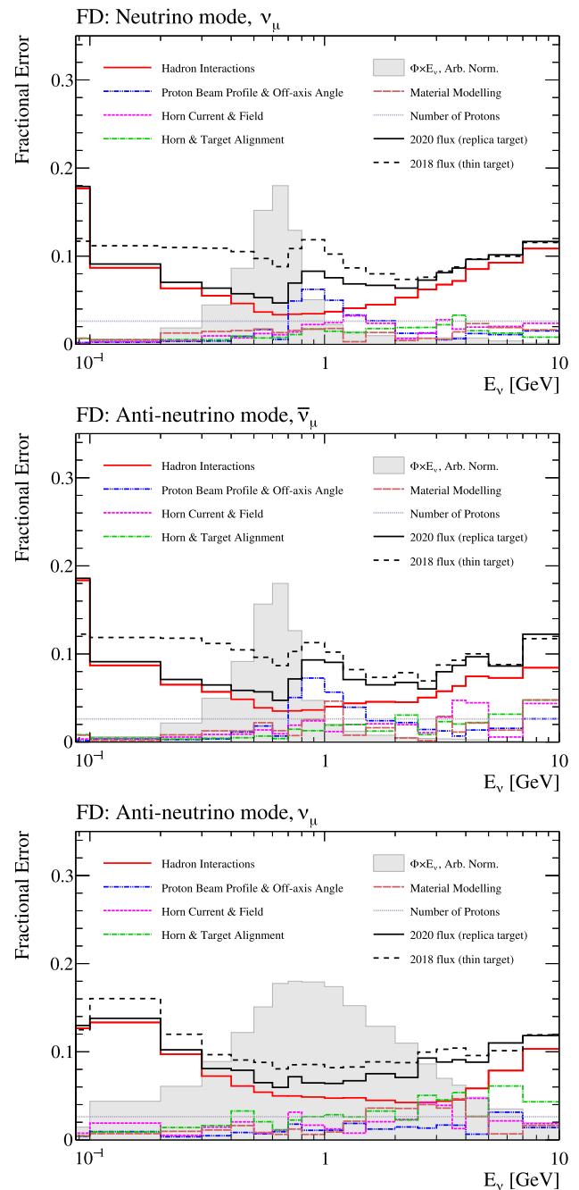
Fig. 6 Uncertainty on the right-sign flux in \nu -mode (top) and right- (middle) and wrong- (bottom) fluxes in \bar{\nu} -mode, broken down by the sources of uncertainty. The solid black line shows the total flux uncertainty in this analysis, and the dashed black line shows the total uncertainty for the previous T2K analysis [1, 2], which used NA61/SHINE thin target data. The grey shaded region shows the shape of the neutrino flux
