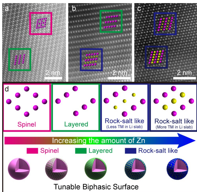
Figure 3. (a-c) STEM-HAADF images to show the surface structure of samples with the increase of Zn content. (a) Coexistence of a spinel phase and a layered phase. (b) Coexistence of the layered phase and the rock-salt like phase. (c) Surface dominated by rock-salt like phase at high Zn content. (d) Schematic illustration for the phase evolution observed on LNMO surface in response to the change in Zn content. The spinel surface will be transformed into different phases with a highly tunable phase ratios, which highlights a gradual increase of the rock-salt phase in the biphasic layer until its dominance on the surface at high Zn content.
