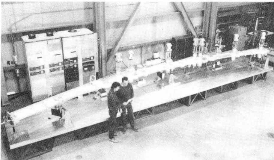
Fig. 2. Twelve of these curved vacuum chambers will be interspersed with twelve straight sections to form the complete storage ring.
