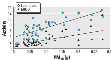
Figure 4. Relationships between PM 10 gravimetric weight and bioassay activities. EROD units, pmol/min/mg protein; r = 0.60^{**} . Luciferase units, RLU × 10 -2 /mg protein; r = 0.76^{**} . Each data point represents the mean of four replicates. ** Significant difference from zero at p < 0.001 level.
