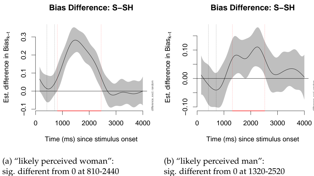
Figure 3.21: Model predicted Bias_{k-t} difference between S and SH C1 steps for intermediate C2 step. The bolded red regions indicate areas in which the Bias difference is significantly different from zero. The vertical dotted lines indicate the beginning of C2 and the end of the stimulus, shifted 150ms forward to account for delays in programming eye movements.
