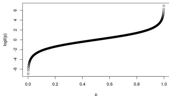
Figure 2.2: Logit-Link Function.
