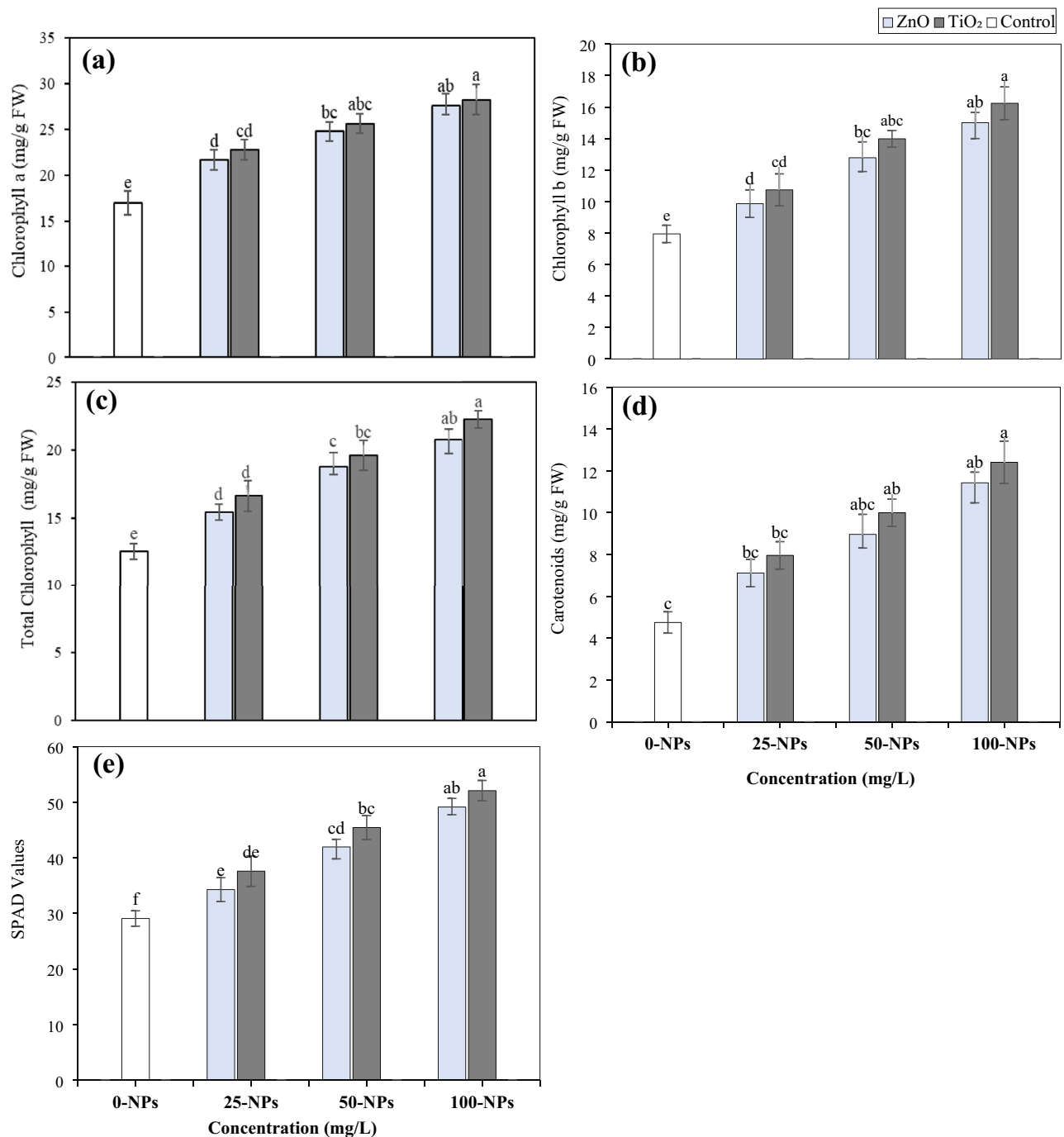
Figure 5. Effect of ZnO-NPs and TiO 2 -NPs on chlorophyll a (a), chlorophyll b (b), total chlorophyll (c), carotenoids (d) and SPAD values (e) of Brassica napus L. grown under lead contaminated soil. The vertical bar on the graph demonstrates the standard deviation. Data are presented as mean \pm SD (n = 3). Different letters on the bars indicate significant differences among treatments at p \leq 0.05 .
