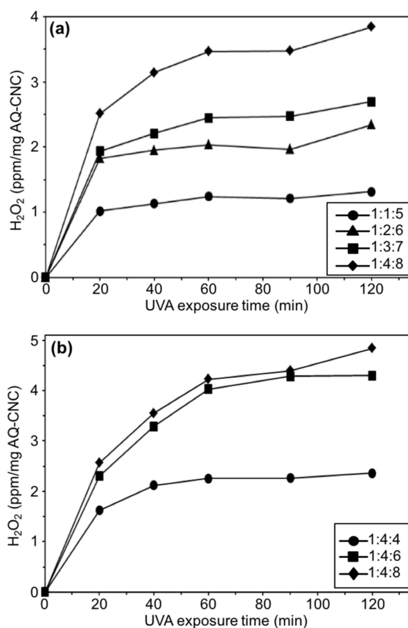
Figure 5. Amounts of hydrogen peroxide produced under UVA (a) by AQ-CNCs made from varied AGU/AQC molar ratios at a reaction time of 2 h and (b) by AQ-CNCs made from varied AQ/CDI molar ratios at a reaction time of 24 h.
