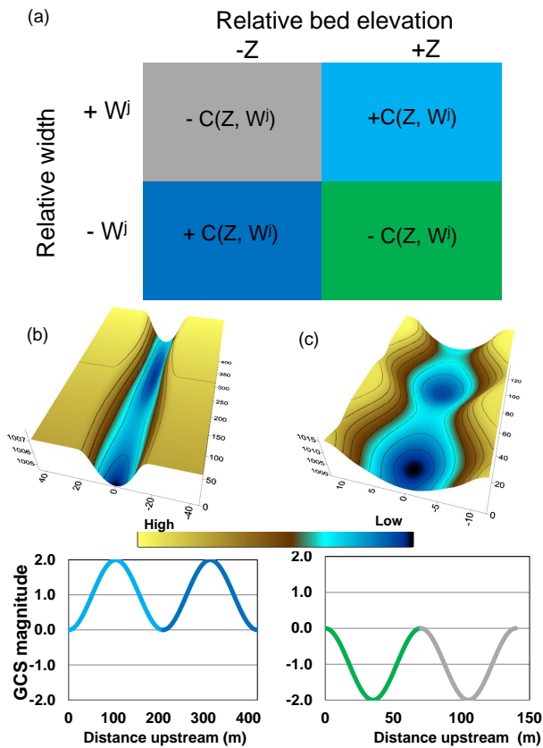
Figure 3. Conceptual key for interpreting C(ZW^j) geomorphic covariance structures (a). For quadrant 1, Z and W^j are both relatively high, so that implies wide and shallow areas associated with deposition. Conversely, in quadrant 2, Z is relatively low, but W^j is relatively high, which implies deep and wide cross areas, which in turn implies that these areas may have been scoured at larger flows. In quadrant 3, Z and W^j are both relatively low, so that implies narrow and deep areas associated with erosion. Finally, in quadrant 4, Z is relatively high and W^j is relatively low, so that implies narrow and topographically high areas. Prototypical channels and GCS with positive (b) and negative (c) C(ZW^j) colored according to (a).
