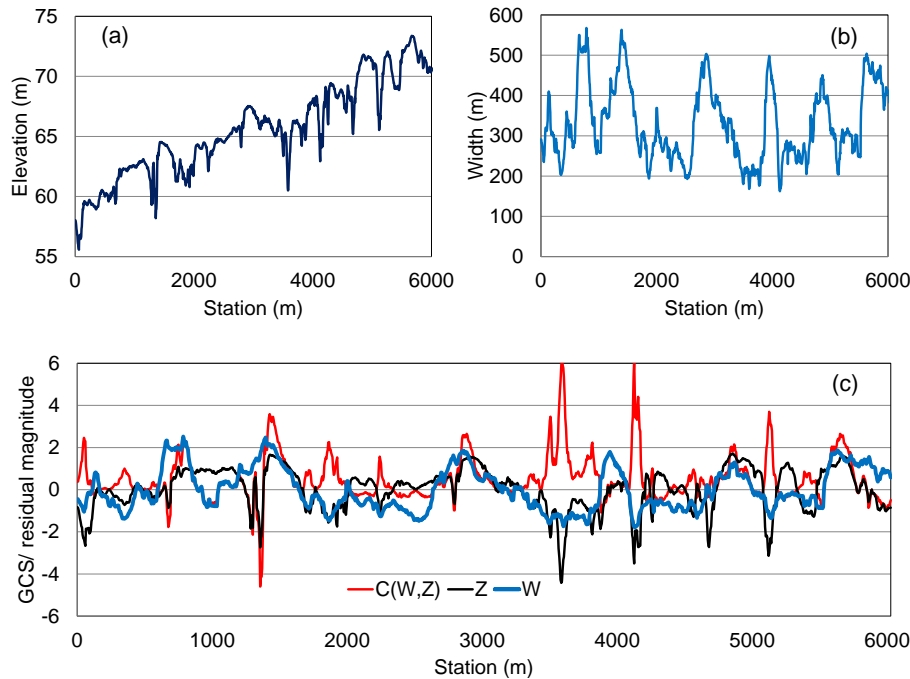
Figure 2. Raw bed profile (a) and flow width (b) series for 283.2 \text{ m}^3 \text{ s}^{-1} . After detrending and standardizing, values of Z (black line in c) and W (blue line in c) are multiplied together to compute C(ZW^j) (red line in c). The whole series of C(ZW^j) is the GCS.
