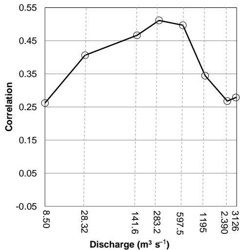
Figure 7. Pearson's correlation coefficient for Z and W^j between each flow.
