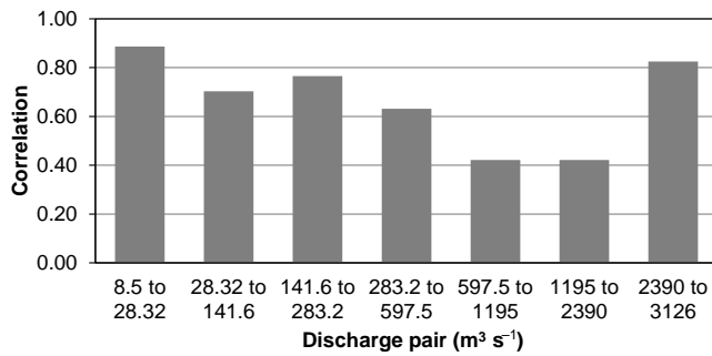
Figure 8. Pearson's correlation coefficient for sequential pairs of flow-dependent wetted width series.
