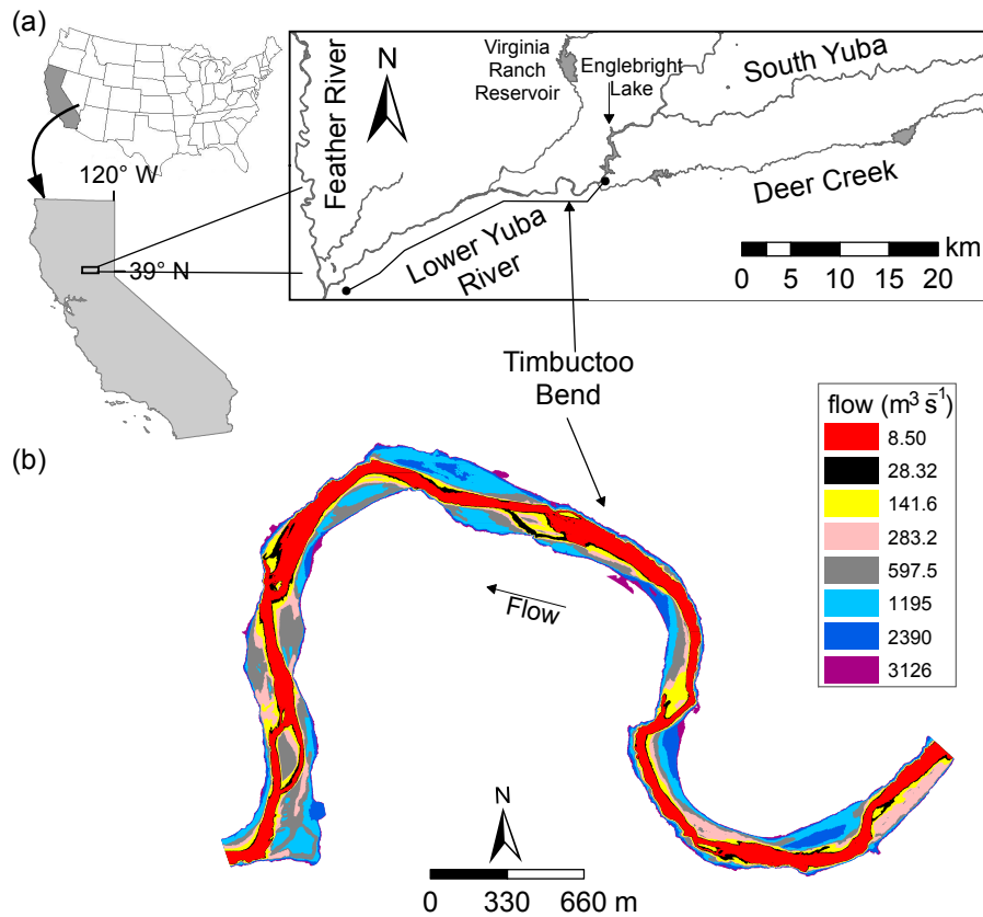
Figure 1. Regional and vicinity map of the lower Yuba River (a) and extent of study segment showing inundation extents predicted by the 2-D model (b).
