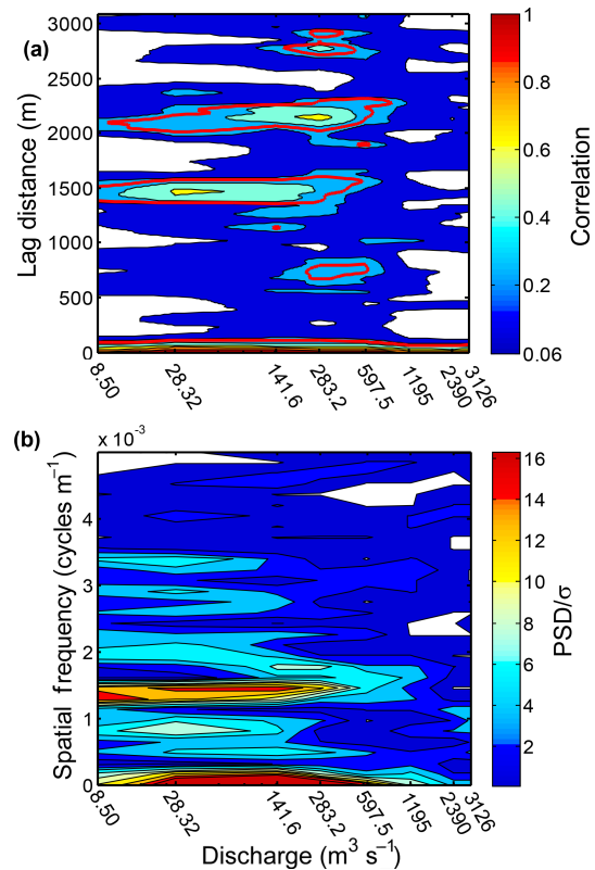
Figure 9. Autocorrelation (a) and PSD (b) of C(ZW^j) with increasing flow. For the ACF plot (a), only values exceeding white noise at the 95 % level are shown and the red contour demarcates the 95 % level for an AR1 process (red noise). For the PSD plot (b) only values exceeding white noise at the 95 % level are shown.
