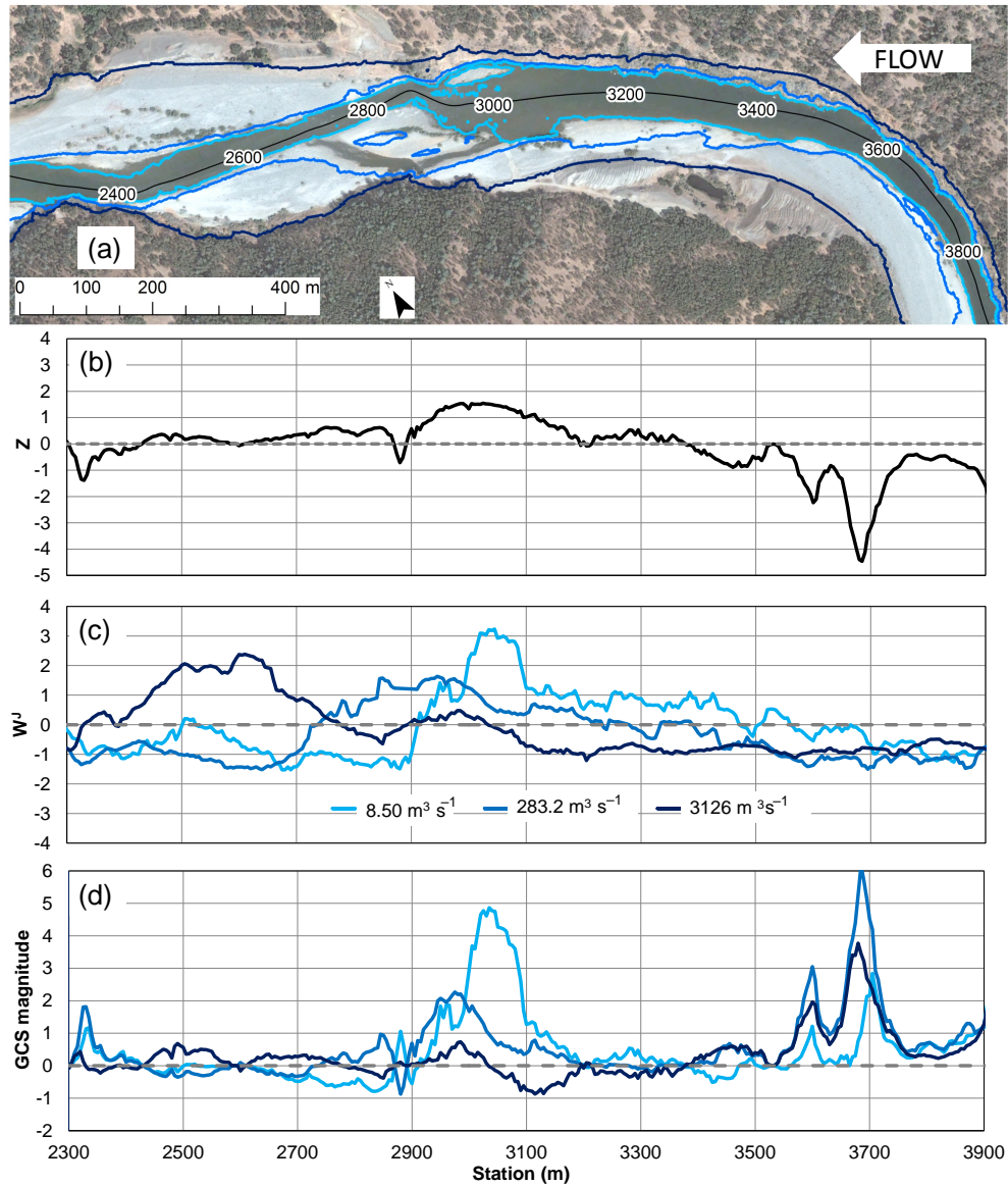
Figure 5. Example section at the lower extent of the study area showing inundation extents (a). Below are plots of minimum bed elevation (b), flow widths for 8.50, 283.2, and 3126 m 3 s -1 (c), and C(ZW^j) for the same flows. The aerial image is for a flow of 21.29 m 3 s -1 on 28 September 2006.
