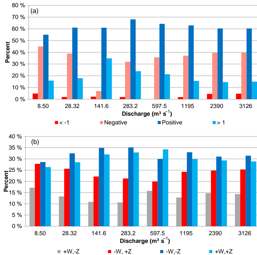
Figure 6. Histogram of C(ZW^j) classified by positive and negative values as well as > 1 and < 1 (a). Also shown is a histogram classified by quadrant (b). The top histogram (a) illustrates the dominance of values C(ZW^j) > 0 regardless of discharge and also illustrates an increasing tendency towards positive values of C(ZW^j) > 1 up until 141.6 \text{ m}^3 \text{ s}^{-1} , after which it declines. The bottom histogram (b) illustrates the distribution of the four quadrant types shown in Fig. 3, with shallow and wide (e.g., +W, +Z ) and deep and narrow (e.g., -W, -Z ) zones being most dominant at 283.2 \text{ m}^3 \text{ s}^{-1} . Colors represent bin-centered values.
