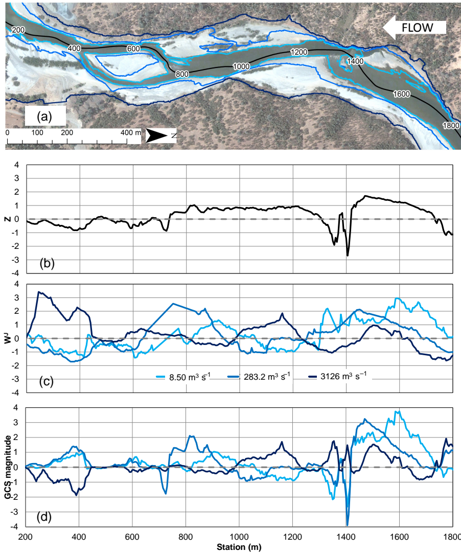
Figure 4. Example section in the middle of the study area showing inundation extents (a). Below are plots of minimum bed elevation (b), flow widths for 8.50, 283.2, and 3126 \text{m}^3 \text{s}^{-1} (c), and C(ZW^j) for the same flows. The aerial image is for a flow of 21.29 \text{ m}^3 \text{s}^{-1} on 28 September 2006.
