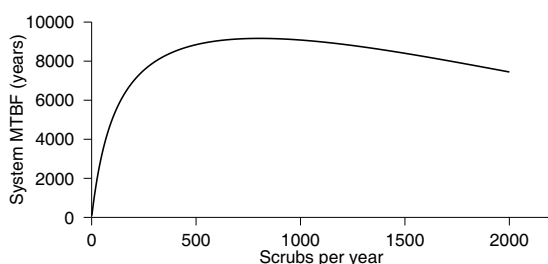
(b) Mirrored disks using opportunistic scrubbing.
