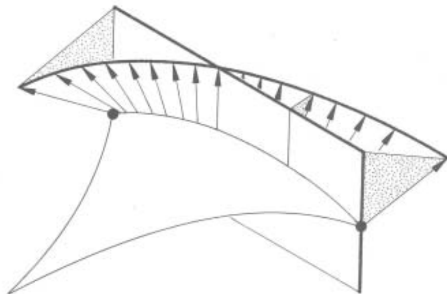
FIG. 6.3. Generating surface normal along edge e_i .
