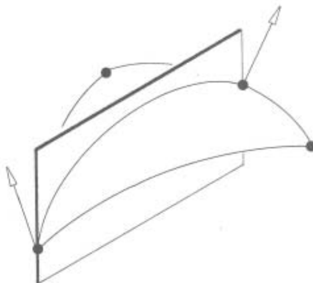
FIG. 6.4. Evaluating surface building block s_i(u) .
