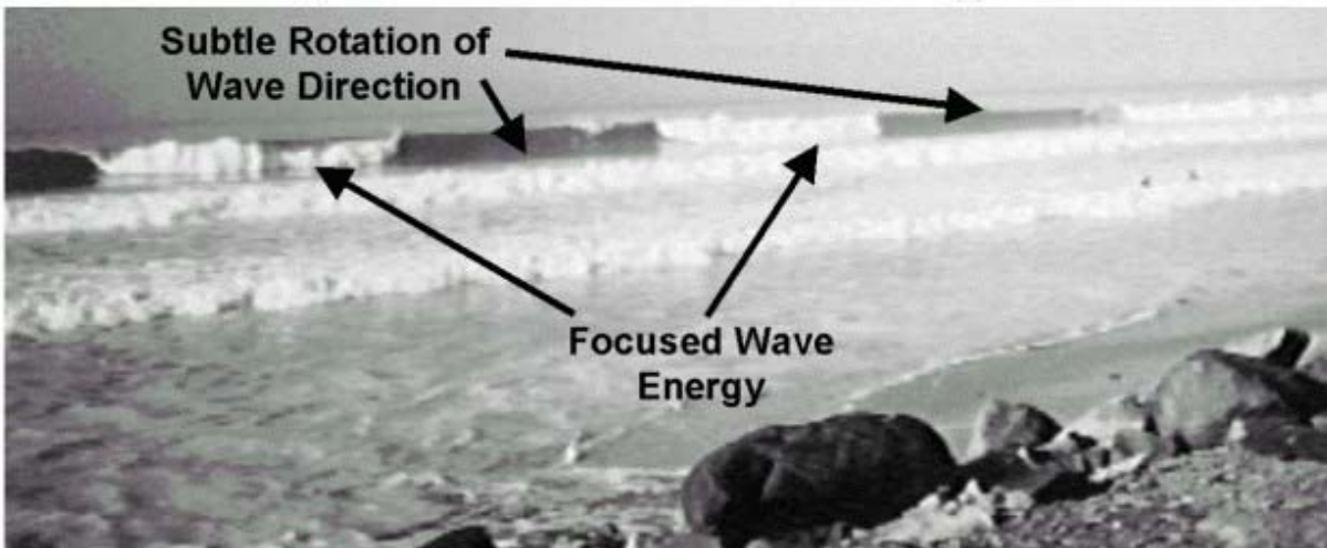
Figure 8. Refraction predictions and image of peeling surfing waves at Tamarack. The modeled wave is 1.5 m, 14 s from 240° (model grid direction -0°). Short peeling waves form because of subtle focusing and rotation of waves.
