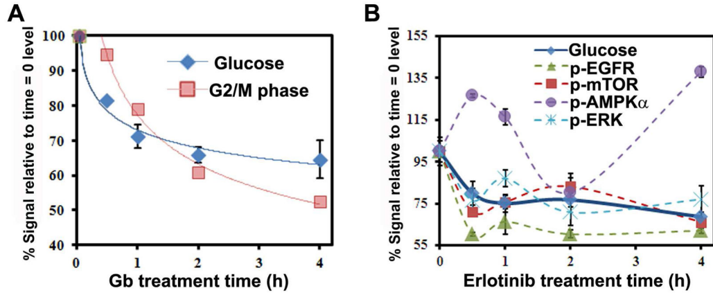
Figure 3. Betabox assays, correlated with other functional assays, for gauging the response of cancer cells to targeted drugs. For these plots, the y-axis is % of the initial level (defined at the time =0 point) to allow for all data to be co-represented on the same plots. (A) The kinetics of [ 18 F]FDG uptake and cell cycle arrest (measured using flow cytometry) following gemcitabine treatment of L1210-wt leukemia cells. The solid lines are first order kinetic fits. (B) The kinetics of [ 18 F]FDG uptake compared with the dynamics of phospho-protein levels within the RTK signaling pathway of U87 EGFRvIII PTEN GBM cells upon erlotinib treatment. The lines connecting the data points are to guide the reader. Error bars indicate average values from three repeat assays.
