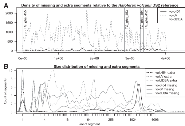
Fig. 1. (A) Density of extra and missing segments in the assemblies of H.volcanii DS2. Reference genome coordinates are given on the x-axis, and red vertical bars delineate the boundaries of the five circular replicons in the reference genome. (B) Size distribution of missing and extra segments in each assembly. The size of a missing segment is given on the x-axis, and the count of missing segments at that size on the y-axis.
