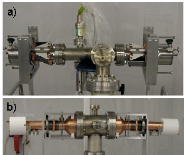
Figure 5: a) Cold and b) Warm Coupler Bake Assemblies at Daresbury
