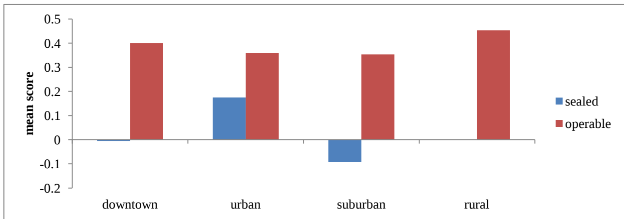
Figure 5 -- Noise satisfaction averages by land use density, n = 19,530.
