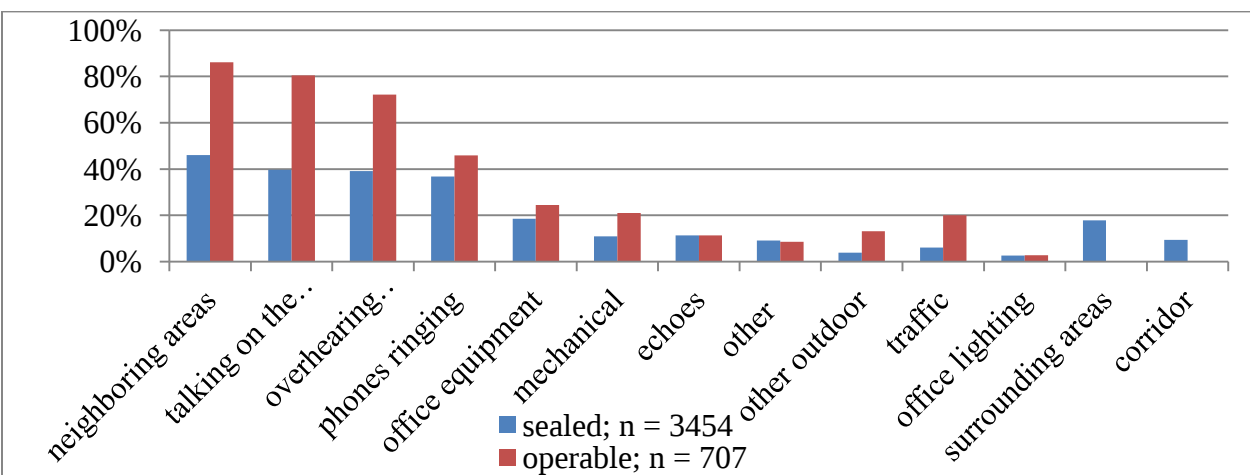
Figure 7 -- Near window sources of noise dissatisfaction.
