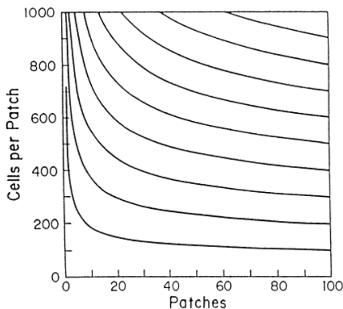
FIGURE 3. Capacity of CA1 model incorporating temporal LTP induction rule. Each contour line denotes an additional 5 million random sequences of length 10, learned in a network composed of a given number of patches each comprising a given number of cells per patch.
