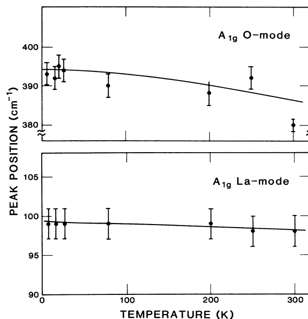
FIG. 3. Peak position of the oxygen A_{1g} mode and the lanthanum A_{1g} mode as a function of temperature.
