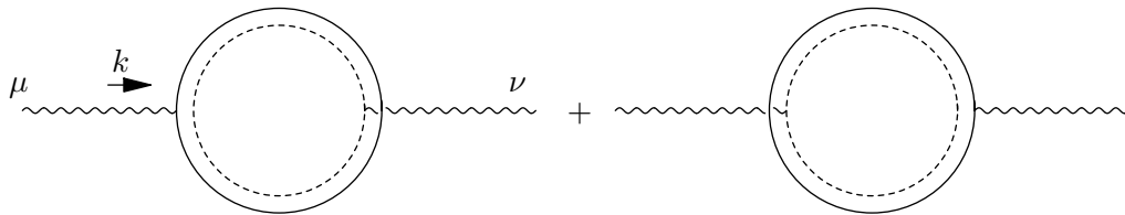
Figure 6: Nonplanar one-loop Feynman diagrams for vacuum polarization.
