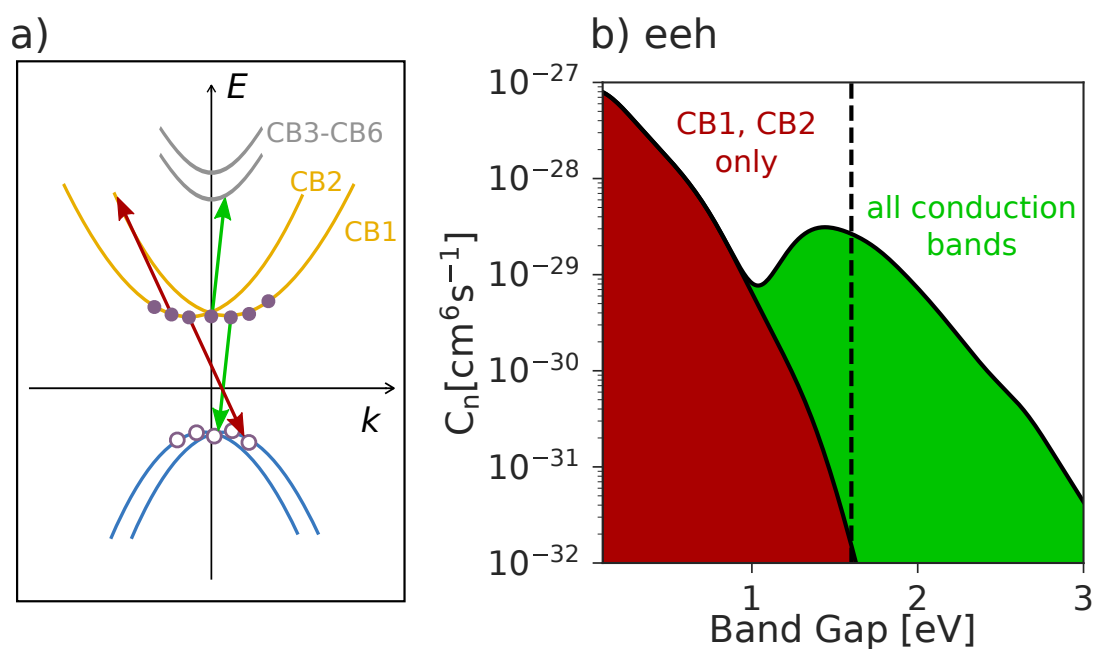
Figure 3. a) Schematic of Auger processes involving only the CB1-CB2 bands vs. processes with transitions to the CB3-CB6 bands. b) Computed Auger coefficients as a function of scissors-adjusted band gap at a carrier density n = 10^{18} \text{ cm}^{-3} , for processes restricted to CB1-CB2 versus processes with transitions to all conduction bands bands. The dashed line represents the experimental band gap of 1.60 eV.
