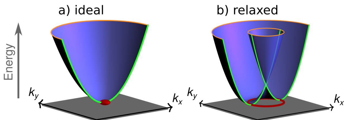
Figure 4. Schematic of the CBM energy dispersion of \text{MAPbI}_3 near the R point for a) the ideal and b) the relaxed structure. The band-edge states are shown in red.
