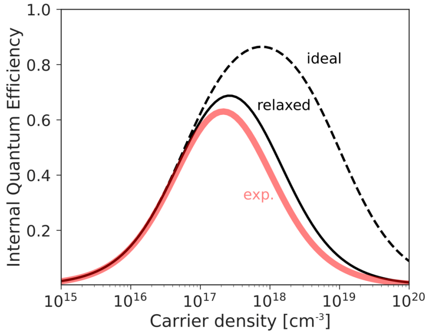
Figure 7. Internal quantum efficiency calculated as a function of carrier density (Equation 1) using k_3 values corresponding to our calculated Auger coefficients for the relaxed (solid curve) and ideal (dashed black curve) perovskite structures, and compared to experimental values.
