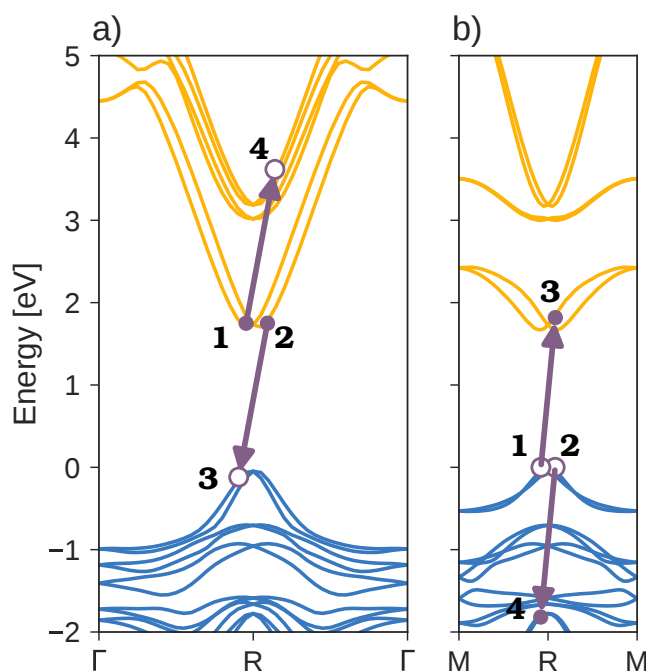
Figure 2. Band structure of MAPbI 3 including SOC, with the gap adjusted to the experimental value, plotted along the a) R \rightarrow \Gamma and b) R \rightarrow M directions. Auger recombination events for the eeh a) and hhe b) processes are indicated.
