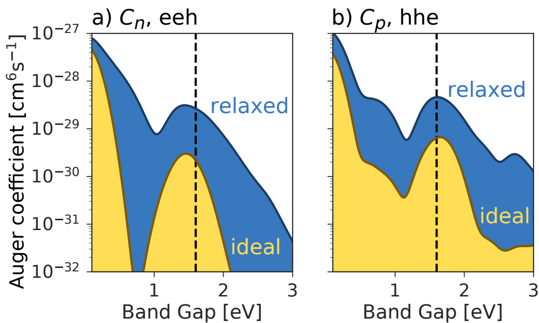
Figure 5. a) eeh and b) hhe Auger coefficients vs. scissored band gap for the ideal and relaxed structures.
