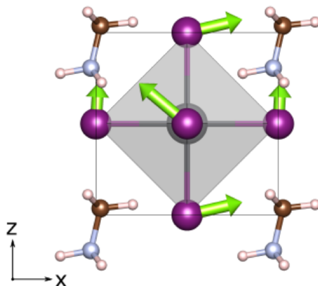
Figure 1. 12-atom unit cell of MAPbI 3 where the I atoms are at the ideal face-center positions. The arrows indicate displacement of the I atoms upon relaxation within a cubic cell shape. For clarity the length of the displacement vector is enhanced by a factor of five.
