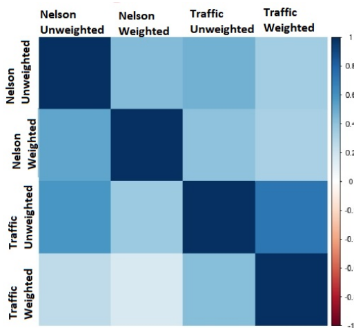
Figure 2: Correlation analysis of the various network representations. The upper diagonal captures Kendall’s tau rank correlation of node degrees across networks. The lower diagonal captures the Pearson correlation between edge weights across the network representations.
