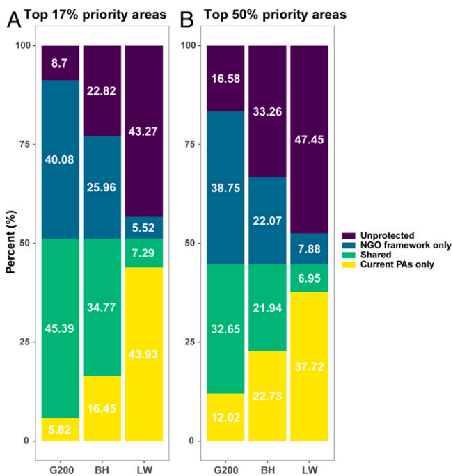
Fig. 5. Percentages of the (A) top 17% and (B) top 50% priority areas for tree conservation covered by existing PAs or by each NGO framework (G200, BH, and LW) for global biodiversity conservation. Colors indicate overlaps between combinations. Unprotected: areas not overlapping with either PAs or a conservation priority framework; NGO framework only: areas overlapping only with the considered NGO framework; shared: areas overlapping with both PAs and a given NGO framework; current PAs only: areas only overlapping with PAs. Priority areas for tree conservation are jointly defined according to taxonomic, phylogenetic, and functional diversity.
