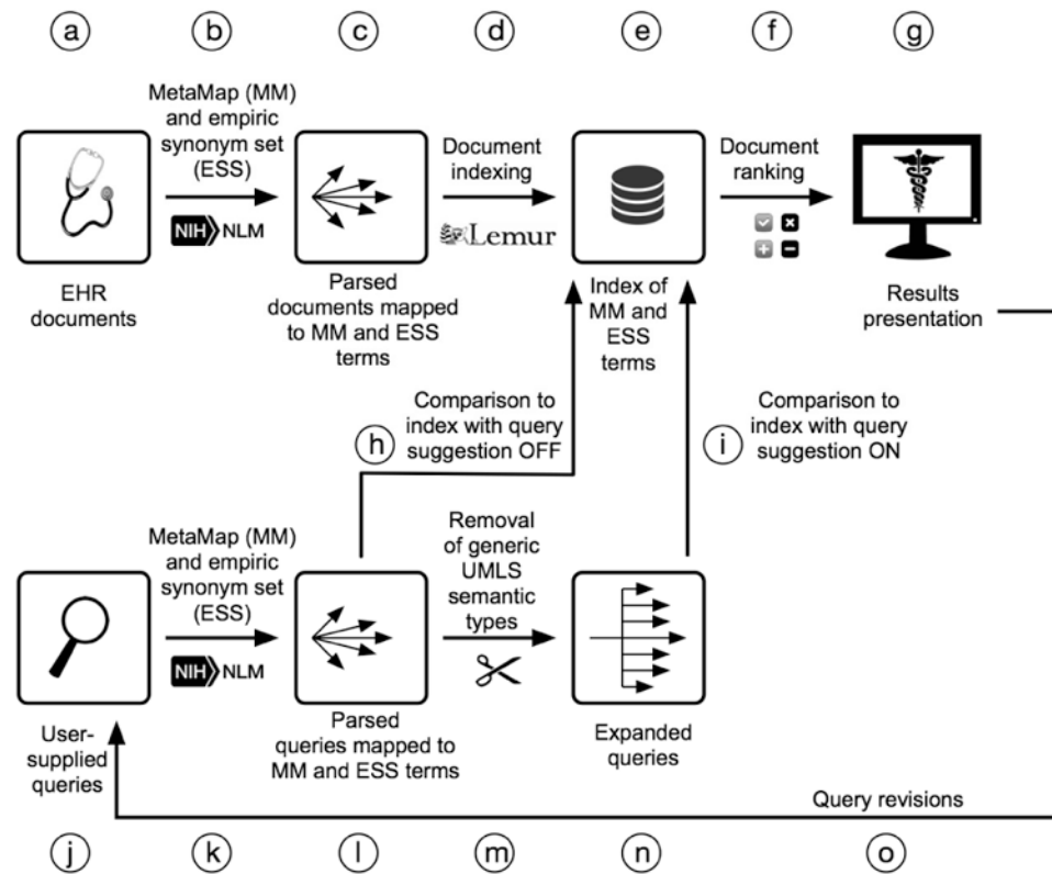
Figure 1. Components and Information Flow of the Query Recommendation Algorithm
