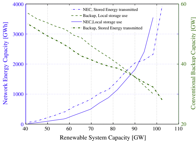
Fig. 6. Network energy capacity (left) and Conventional backup capacity (right) requirement as a function of renewable system size.
