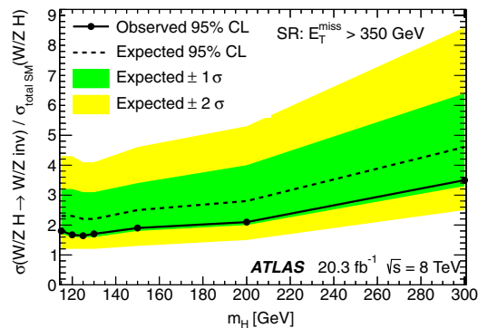
FIG. 6 (color online). Limit on the Higgs boson cross section for decay to invisible particles divided by the cross section for decays to standard model particles as a function of m_H at 95% C.L., derived from the signal region (SR) with E_T^{\text{miss}} > 350 GeV.
