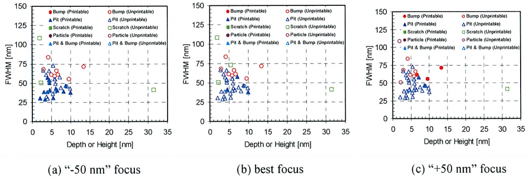
Figure 11. Defect printability as through-focus
