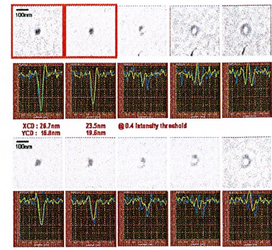
Figure 10. Printability of defects of similar sizes and pit defects
