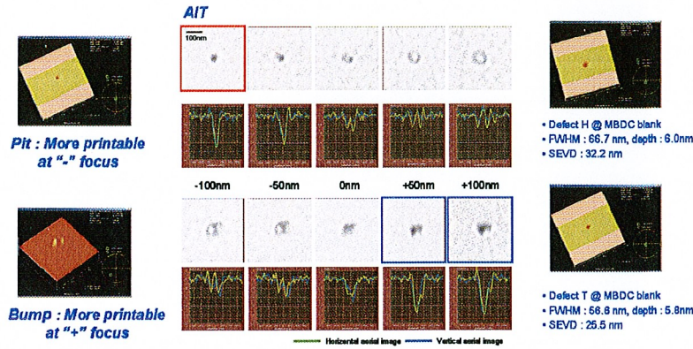
Figure 9. Printability as through-focus of bumps and pits
