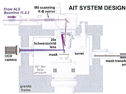
Figure 4. AIT system design
