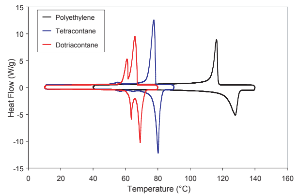
FIG. 2: DSC of polyethylene (black), purified tetracontane (blue), and dotriacontane (red). The sharp peaks are indicative of crystalline phase transitions.
