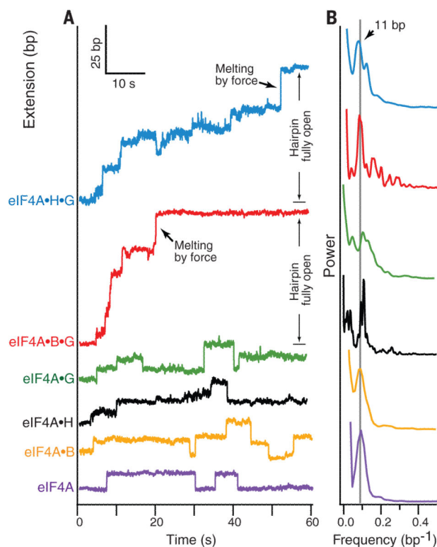
Fig. 2. Factor-dependent processivity of eIF4A
