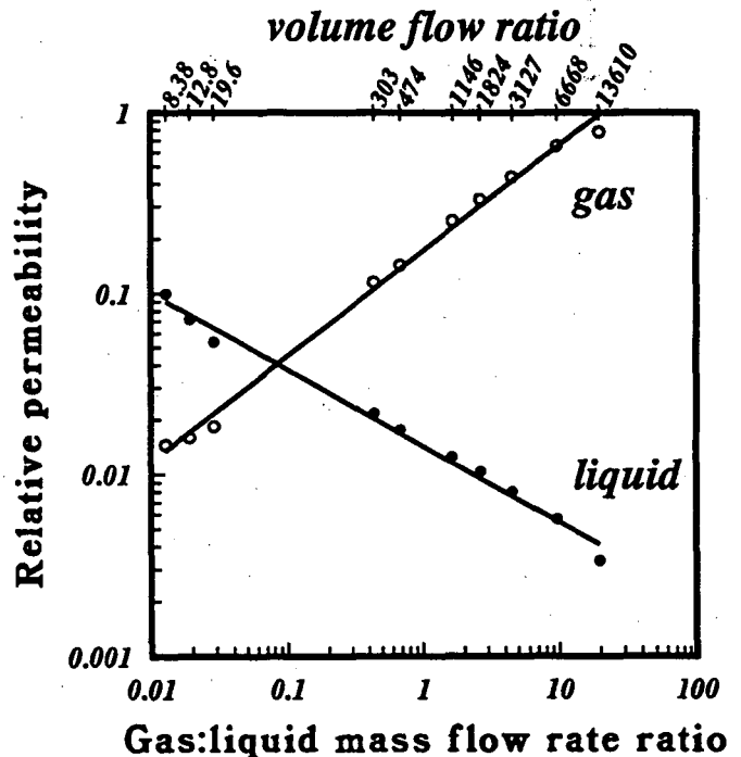
Figure 6. Relative permeability curves calculated from data of Experiment D, Dixie Valley fracture replica.
