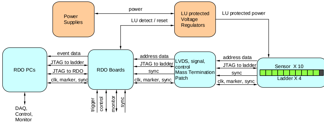
Figure 9 System level functionality diagram of the readout of the PIXEL sensors. One of ten parallel readout chains in shown.
