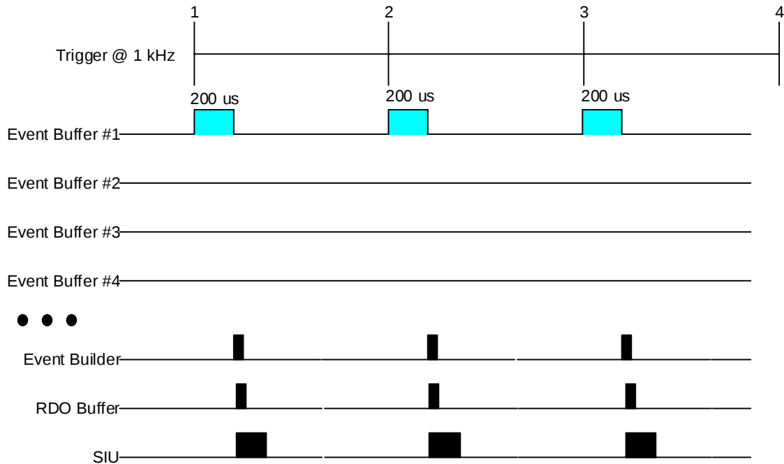
Figure 17 Chronogram of the Ultimate sensor based readout system functions for a 1 kHz periodic trigger.
