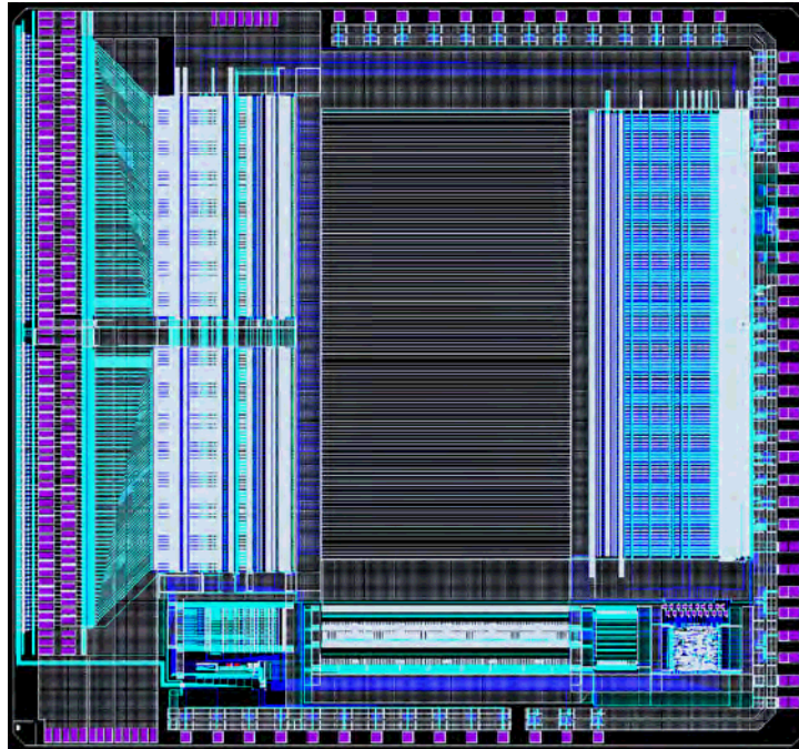
Figure 77: Picture of the APV25-S1 die. On the left are the input pads; on the right are the output pads and control pads. The whole die measures 8.055 by 7.100 mm 2 .
