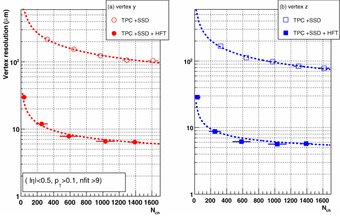
Figure 31: Vertex resolution \sigma(\text{MC Vertex Position} - \text{Reconstructed Vertex position}) as a function of N_{ch} , the number of charged tracks in the reconstructed event. The PIXEL refit vertex shows an order of magnitude improvement over the previously reconstructed primary vertex. a) Vertex resolution in y vs. N_{ch} . b) Vertex resolution along the beam direction. Best resolution is v_y = 6.5 \mu\text{m} , v_z = 5.5 \mu\text{m} .
