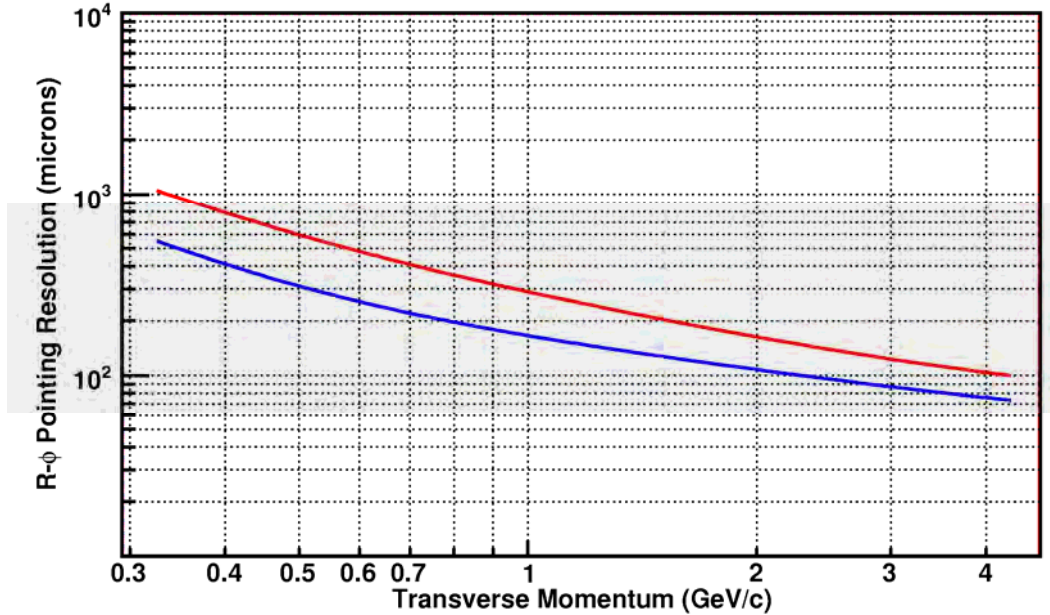
Figure 25: The predicted pointing resolution of the TPC+SSD+SVT at the vertex in the r - \phi direction. The blue line shows the pointing resolution for all three SVT layers. The red line shows the effective resolution if the first layer of the detector is not hit and only layers 2 and 3 have hits.
