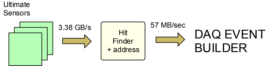
Figure 65: Data rates in ULTIMATE PIXEL readout.
