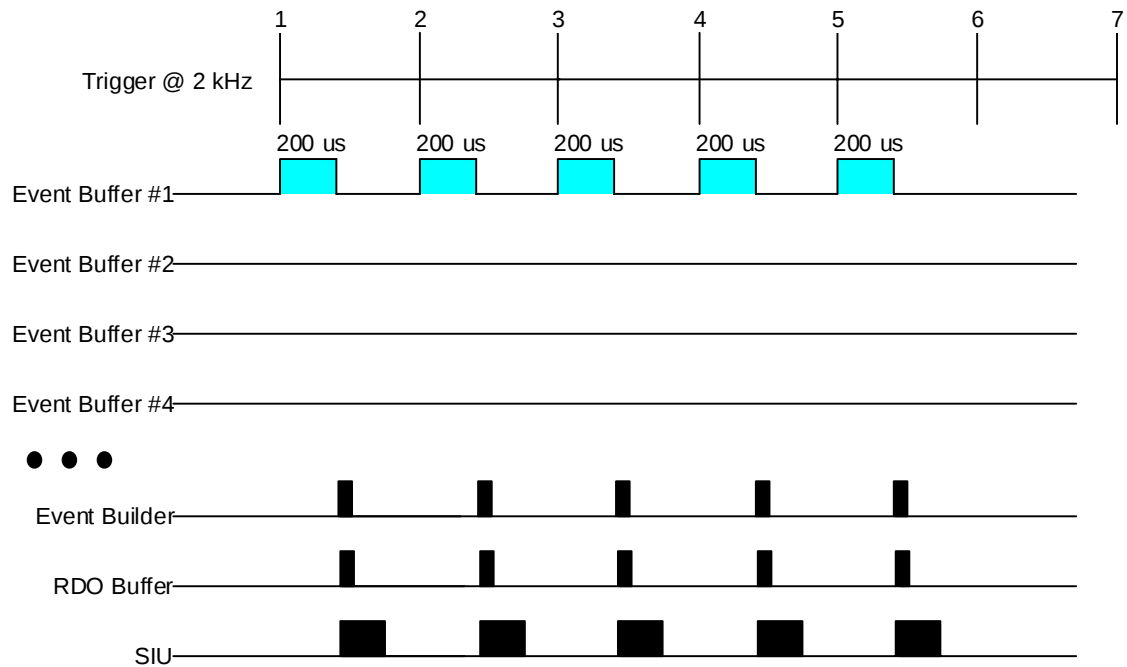
Figure 18 Chronogram of the Ultimate sensor based readout system functions for a 2 kHz periodic trigger.
