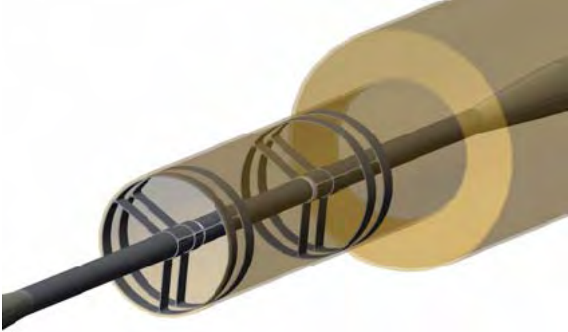
Figure 83: View of the beam pipe mid-section with central support.
