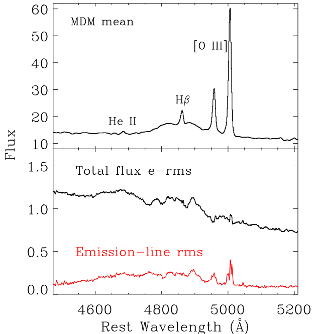
FIG. 2.— The mean and excess rms (Eq. 4) spectra from the MDM dataset are shown in black, and the rms spectrum with the AGN and stellar continuum removed is shown in red (see Section 3.1).
