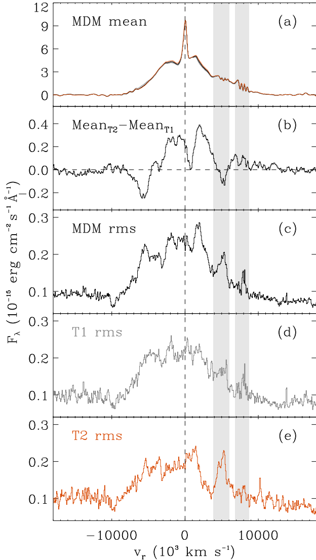
FIG. 5.— The MDM mean spectrum (a), difference between the T1 (THJD < 6747) and T2 (THJD > 6747) mean spectra (b), and the rms spectra (c–e) for H \beta after subtracting all other fit components from spectral decomposition. The colors are for the full campaign (black), T1 (gray), and T2 (orange, see Section 3.3). Zero velocity is determined by the peak of the narrow H \beta line in the mean spectrum, and the gray bands indicate regions contaminated by [O III] residuals. The rms spectra have statistical uncertainties of \sim 12\% .
