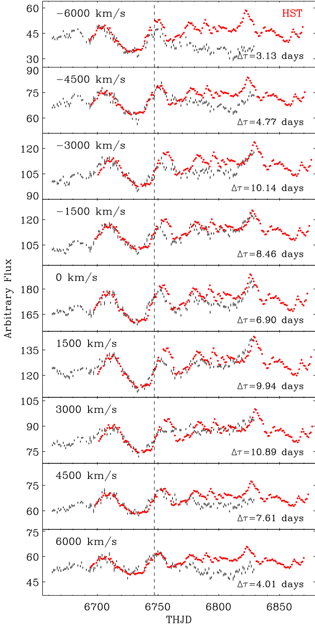
FIG. 11.— Velocity-resolved H\beta light curves for 1500\text{-km s}^{-1} bins (black) with the central velocity for each bin shown at the top left of each panel. HST 1158\text{ \AA} light curves that have been scaled and shifted to match the first half of the H\beta light curves are shown in red, and the dashed line indicates the epoch that separates T1 and T2 for this analysis. The H\beta response to the continuum is distinctly velocity-dependent during the second half of the campaign.
