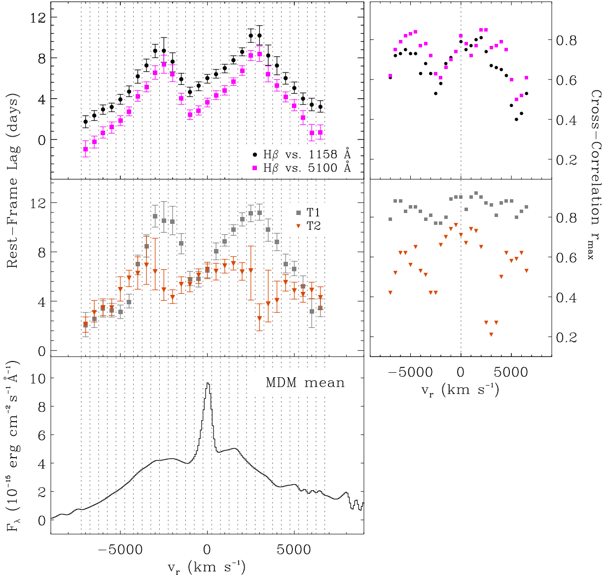
FIG. 10.— Top left: ICCF H\beta lags ( \tau_{\text{cen}} ) for 500-km s^{-1} bins measured against the 1158 \text{\AA} and 5100 \text{\AA} continua. Middle left: Lags for T1 and T2 measured against the 1158 \text{\AA} continuum. Bottom left: MDM mean spectrum for the full campaign. Right: Maximum cross-correlation coefficients ( r_{\text{max}} ) for individual velocity bins.
