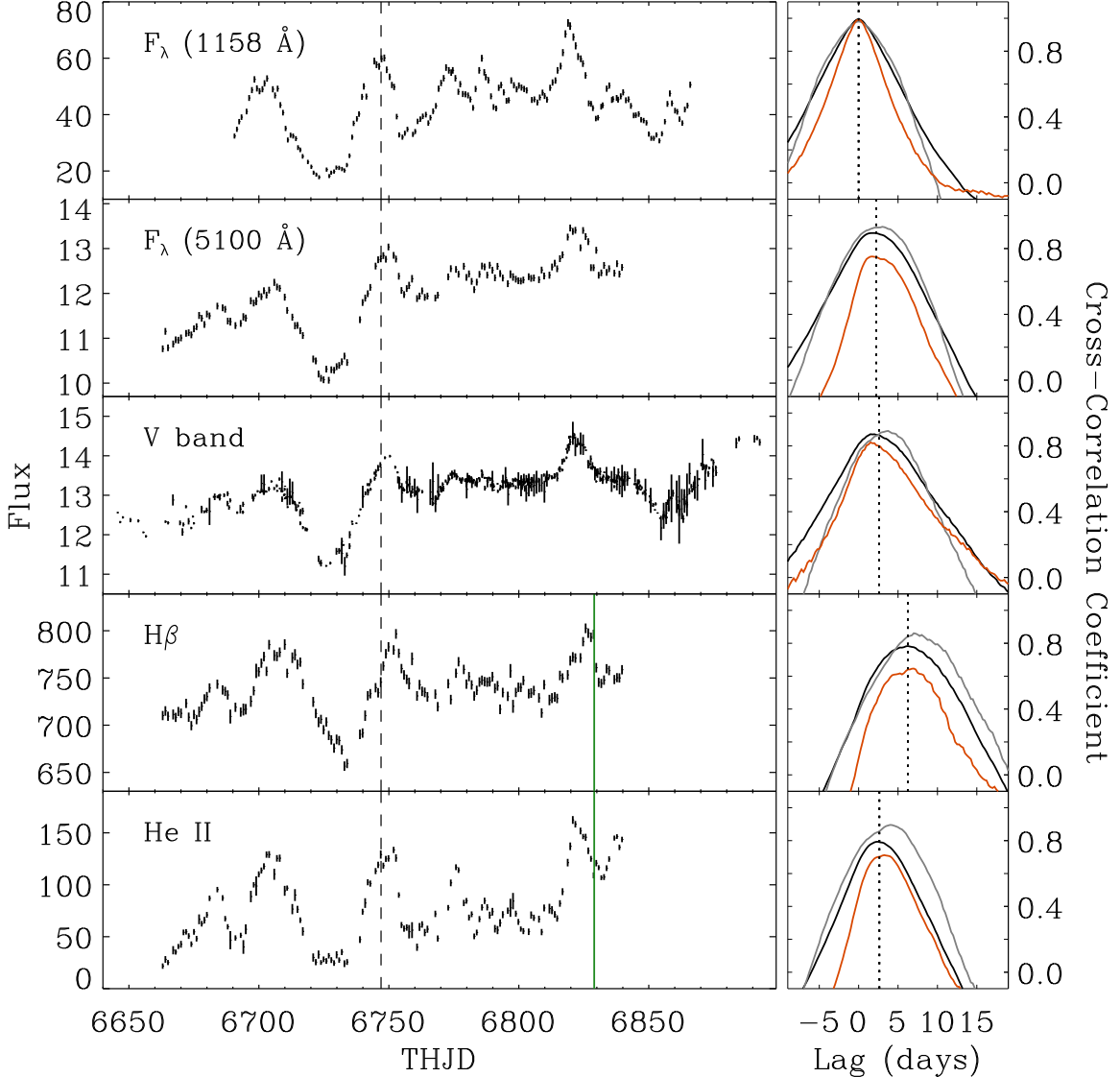
FIG. 6.— Left : Light curves for the UV 1158 Å continuum, optical 5100 Å continuum, V-band continuum, H \beta , and He II \lambda 4686. The continuum light curves are in units of 10^{-15} \text{ erg s}^{-1} \text{ cm}^{-2} \text{ \AA}^{-1} and the line light curves are in units of 10^{-15} \text{ erg s}^{-1} \text{ cm}^{-2} . The H \beta and He II fluxes include contributions from both broad and narrow line components. The H \beta and He II fluxes were truncated for the lag analysis (see text) and the dashed black vertical line shows the division between the T1 and T2 periods. Right : Cross-correlation functions for each light curve measured against the 1158 Å continuum. The top right panel shows the auto-correlation of the 1158 Å light curve. The black, gray, and orange solid lines represent the CCFs for the full campaign, T1, and T2 (respectively), and the dotted vertical lines denote \tau_{\text{cen}} for the full campaign.
