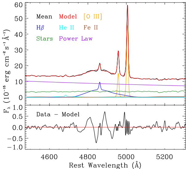
FIG. 4.— Top : Spectral decomposition components of the mean MDM spectrum. The red spectrum is the sum of all model components and traces the data (black spectrum) well over most of the spectral range. Bottom : Residuals from the full model fit.
