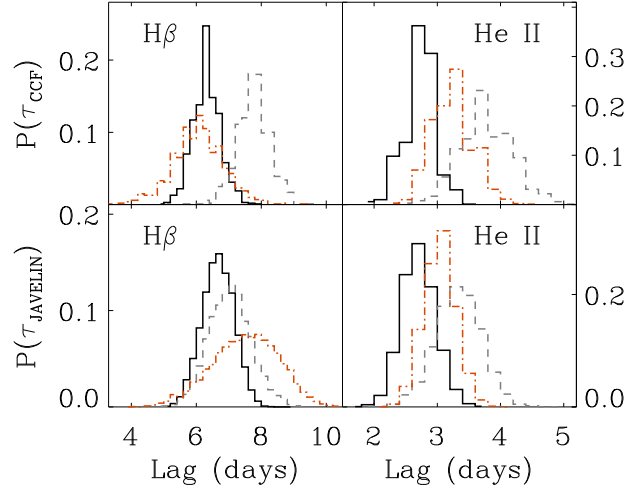
FIG. 8.— \tau_{\text{cen}} (top) and JAVELIN (bottom) lag probability distributions for H \beta (left) and He II (right) measured against the 1158 \text{\AA} continuum. Black solid lines are for the full campaign, gray dashed lines are for T1, and orange dot-dash lines are for T2.
