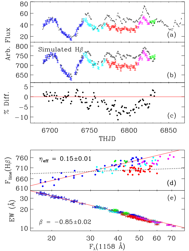
FIG. 12.— Panel (a) shows 1158\text{ \AA} continuum light curve with the time-shifted H\beta light curve (see text for color scheme). Panels (b) and (c) show the reconstructed H\beta light curve (gray dots) and the percent of flux lost during the anomaly, respectively. Panels (d) and (e) show the H\beta broad-line flux ( 10^{-15}\text{ erg s}^{-1}\text{ cm}^{-2} ) and EW ( \text{\AA} ) as a function of the 1158\text{ \AA} continuum flux density ( 10^{-15}\text{ erg s}^{-1}\text{ cm}^{-2}\text{ \AA}^{-1} ). The solid red lines are linear least-squares fits to the blue points, which are from the period when the line and continuum light curves are well-correlated. The slopes of these fits are shown in each panel. The dotted black line in panel (d) is the least-squares fit to the red points (anomaly) and has a slope of \eta_{\text{eff}} = 0.02 \pm 0.03 .
