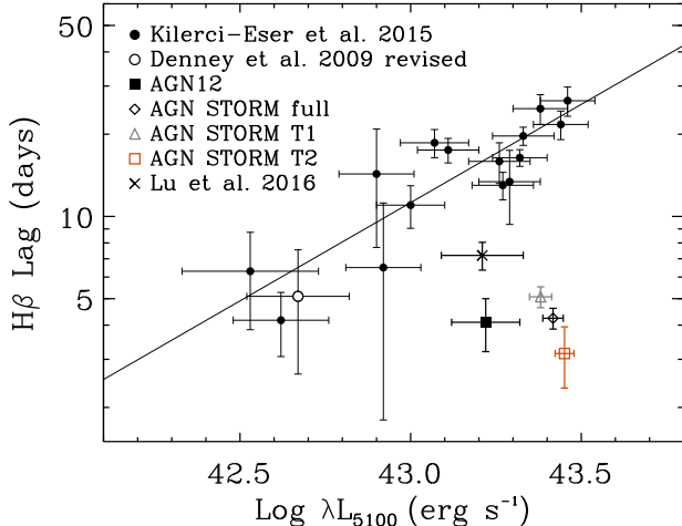
FIG. 13.— NGC 5548 optical continuum luminosity and H\beta -optical lags from all monitoring campaigns to date. The solid line is the linear least-squares fit to the Kilerci Eser et al. (2015) and Denney et al. (2009) points.
