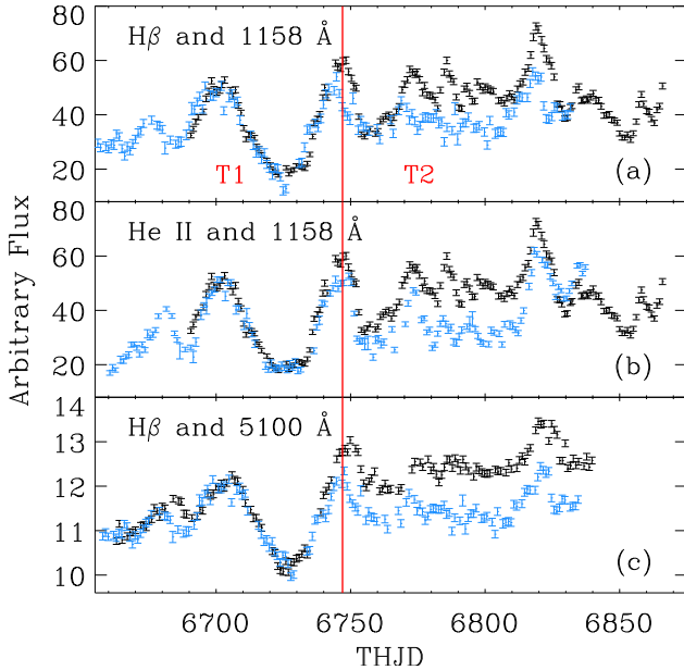
FIG. 7.— 1158 \text{\AA} and 5100 \text{\AA} continuum light curves (black) compared with scaled and shifted emission-line light curves (blue). The vertical line at THJD = 6747 indicates the epoch separating the T1 and T2 segments. In each of the panels, the emission-line light curve closely tracks the continuum light curve in T1, but appears to correlate less closely with the continuum variations in T2.
