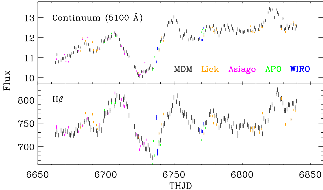
FIG. 3.— Continuum ( 10^{-15} erg s ^{-1} cm ^{-2} Å ^{-1} ) and H \beta ( 10^{-15} erg s ^{-1} cm ^{-2} ) light curves (THJD = HJD - 2,450,000). The Lick, APO, Asiago, and WIRO light curves were scaled and shifted to match the MDM light curve, which has the longest temporal coverage and highest sampling cadence. The plotted uncertainties include Poisson noise and the normalized excess variance of the [O III] light curve (Section 2.1.)
