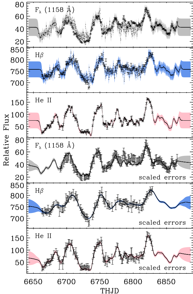
FIG. 9.— JAVELIN light curves from simultaneously modeling the H\beta and He II \lambda 4686 emission lines with the UV 1158 \text{\AA} continuum. The data points are measured from observations, the black solid lines are the weighted means of the model light curves consistent with the data, and the thickness of the shaded regions indicates the 1\sigma spread of those light curves. The top three panels show the observed data and JAVELIN model light curves without any error scaling, and the bottom three panels show the data and light-curve models with scaled uncertainties.
