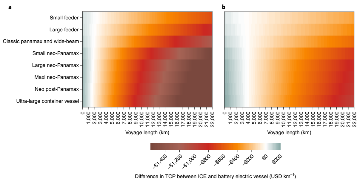
Fig. 4 | Difference in TCP between battery-electric and ICE vessels for all eight size classes for voyages up to 22,000 km. a,b, The baseline (a) and near-future (b) scenarios. TCP excludes environmental costs. A positive value indicates that the TCP of the battery-electric ship is lower than that of the ICE equivalent, whereas a negative value represents a lower ICE TCP. The TCP difference is larger in magnitude for larger ship classes, indicating the difficulty of cost-effectively electrifying large containerships over intercontinental routes, but also the potential economic benefit of phasing in battery-electric vessels over short to medium intraregional routes.
