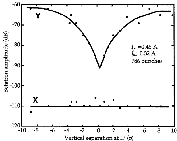
Figure 4: Betatron motion vs beam separation
