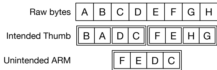
(a) Class 1: First halfword of 32-bit Thumb instruction
