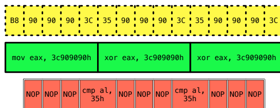
Figure 1.1. Illustration of a NOP sled encoded in the bytes implementing the statement x = 0x3c909090 \oplus 0x3c909090 \oplus 0x3c909090 ;
