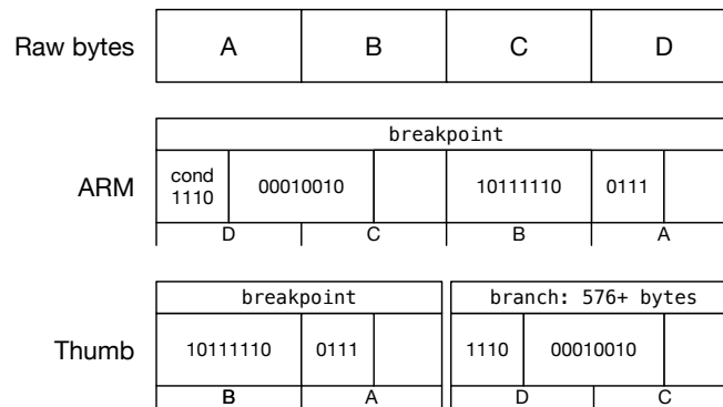
Figure 8.4. Diagram of breakpoint instruction encodings as they might appear in an INSeRT-style trapping snippet on ARM.
