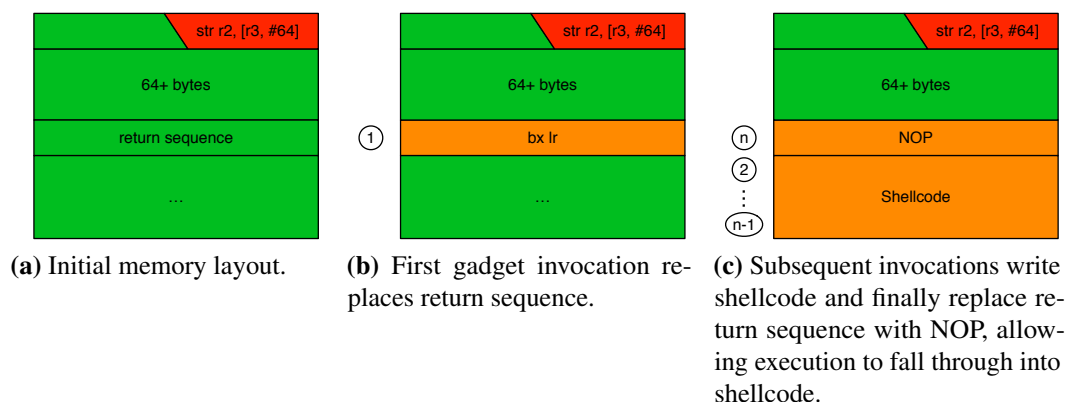
Figure 5.2. Progression of our proof of concept attack's self-modifying code. Encircled numbers to the left show the order in which the self-modifying writes occur.
