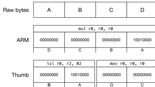
Figure 8.5. Diagram of pseudo NOP instructions that can be used to construct a pseudo NOP sled in an ARM/Thumb trapping snippet.
