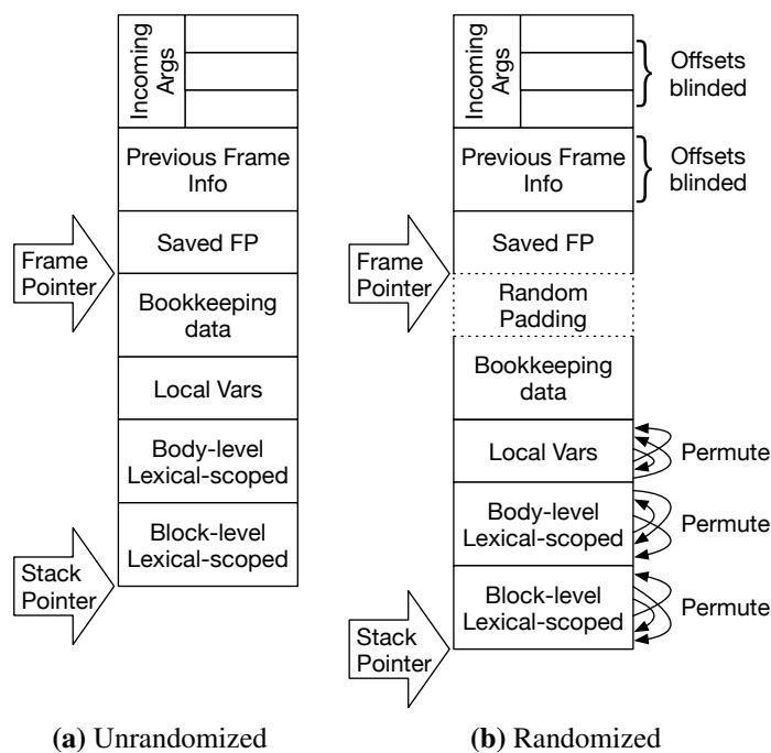
Figure 8.1. Baseline JIT call stacks with and without call frame randomization. Stacks grow downward.
