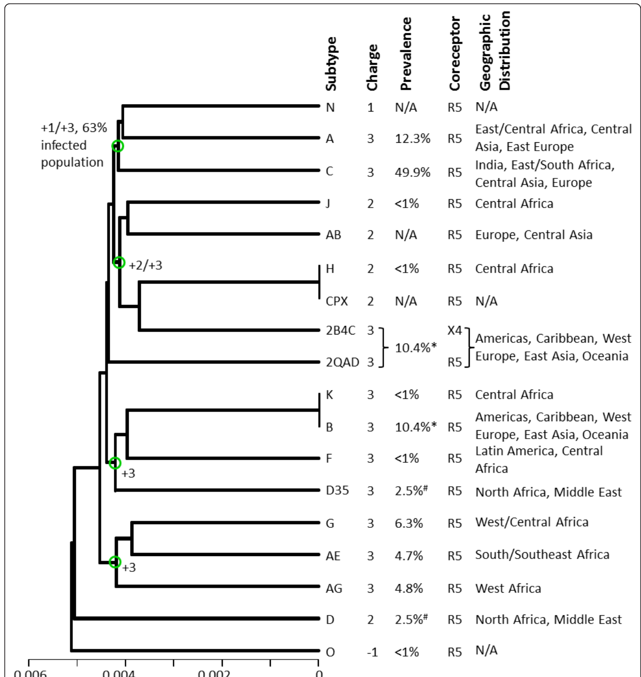
Figure 4 Charge distribution clustering analysis of the HIV-1 subtypes, from the year 2009 consensus sequences and structural template derived from the gp120 structure with PDB Code 2QAD. The horizontal axis of the dendrogram represents charge similarity distance. The net charge, global prevalence, coreceptor selectivity and geographies of each subtype are indicated in the figure for each subtype. N/A denotes that information was not available. Green circles in the branches of the dendrogram denote intersection points between net charges or infected population. The symbol * refers to the global prevalence of Subtype B which includes the two crystal structural templates (from 2QAD and 2B4C). The symbol # refers to the global prevalence of Subtype D which includes D and D35, combined.
