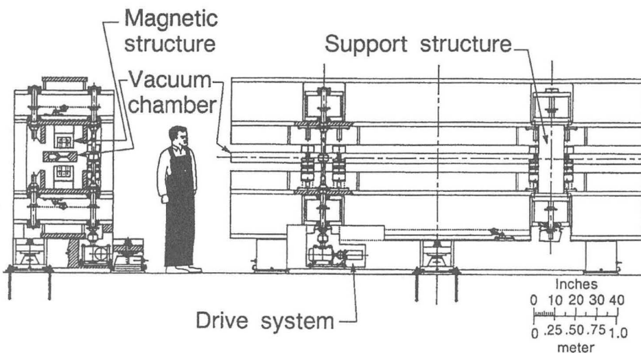
End view
