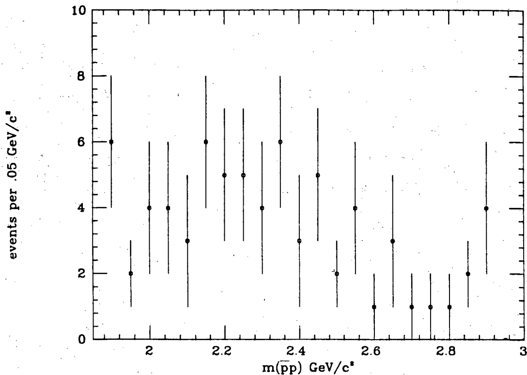
Figure 25: Mass of \bar{p}p pairs opposite direct photons, \pi^0 background unsubtracted. The rise near 2.9 \text{ GeV}/c^2 is probably due to \psi \rightarrow \bar{p}p events coupling with noise photons, as the q^2 cut is not very stringent for low momentum photons.
