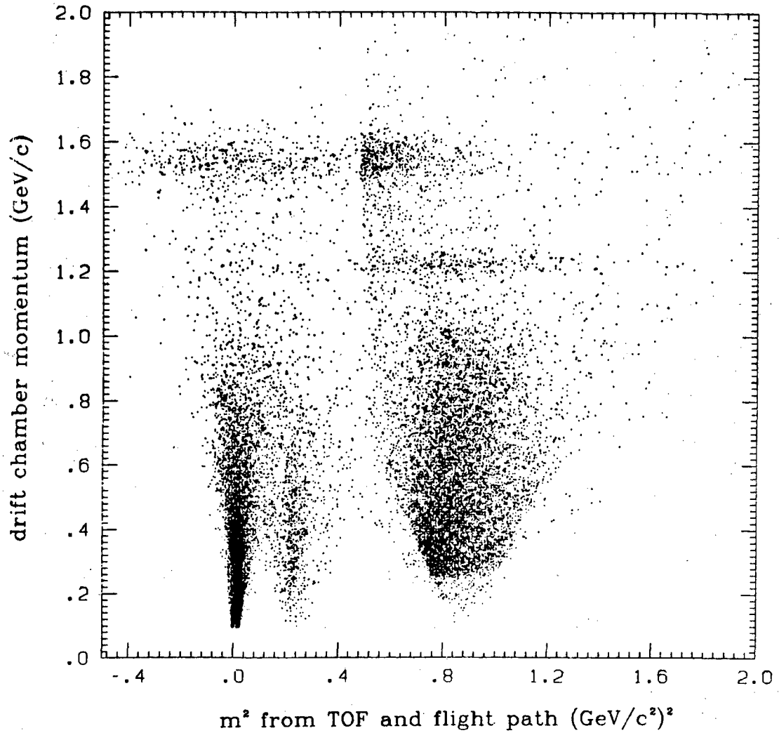
Figure 6: Scatterplot of m^2 vs. momentum. The cutoff near m^2 = .5 \text{ (GeV/c}^2\text{)}^2 is due to a loose proton weight cut on the data sample. This is looser than any other cut on the data samples used in this thesis. The horizontal band structure is discussed in the text.
