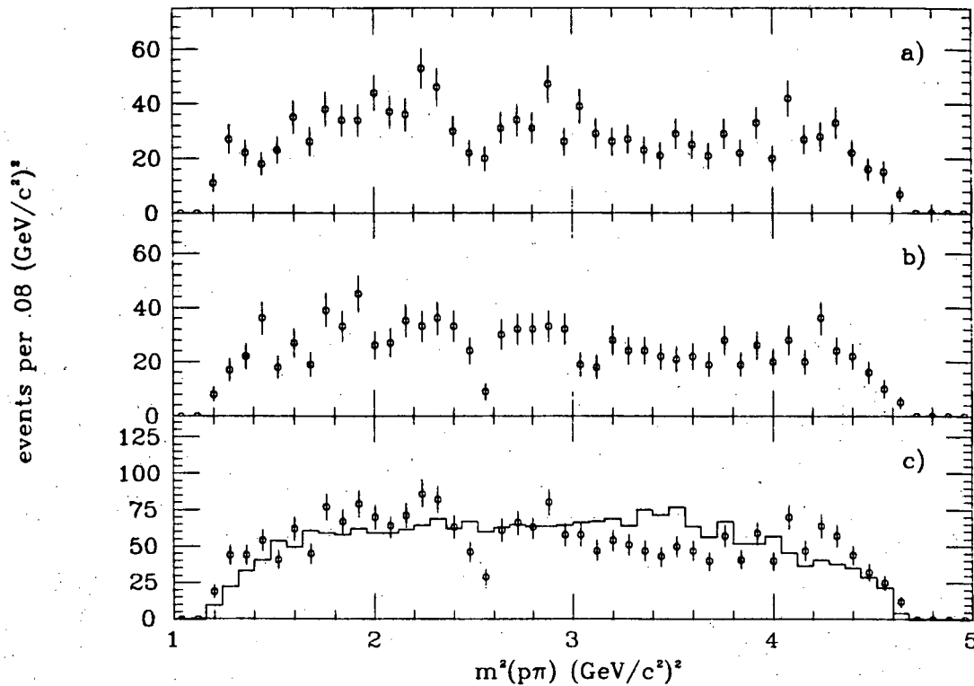
Figure 28: Dalitz projections for \psi \rightarrow \bar{p}\pi^+n + \text{c.c.}
