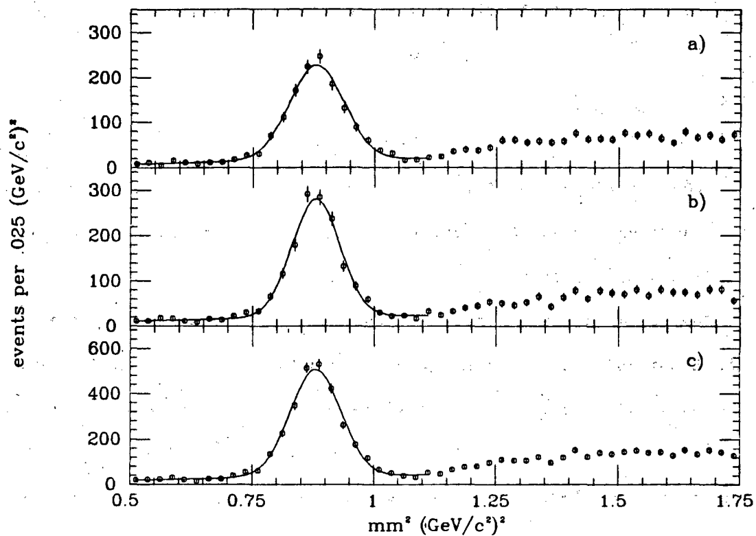
Figure 26: mm^2 against N\pi system.
