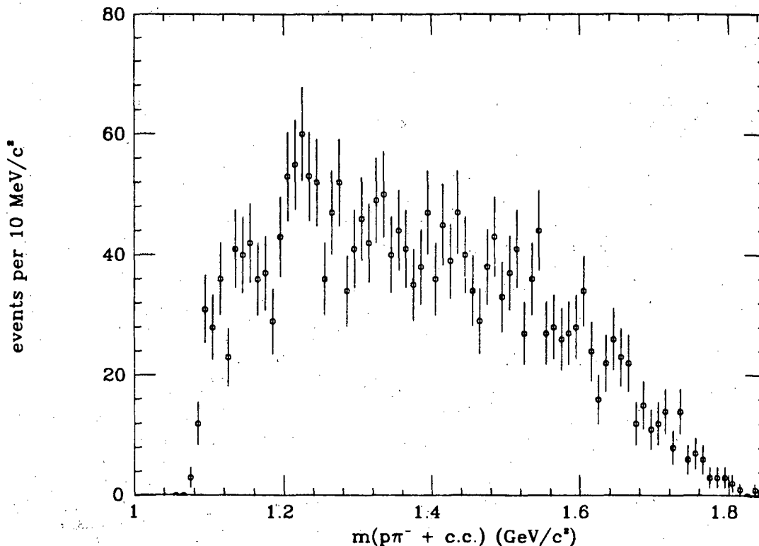
Figure 47: m(p\pi^-) , \Lambda\bar{\Lambda} and \Delta^{++}\bar{\Delta}^{--} subtracted.
