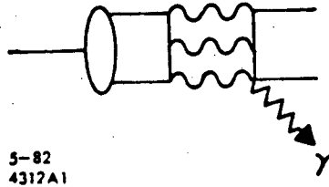
Figure 3: Radiative three gluon decay.
