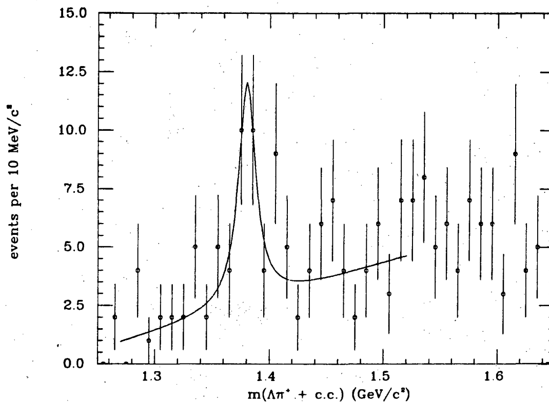
Figure 57: \Lambda\pi^+ + c.c. mass opposite \Sigma recoil. Solid line is fit described in text.
