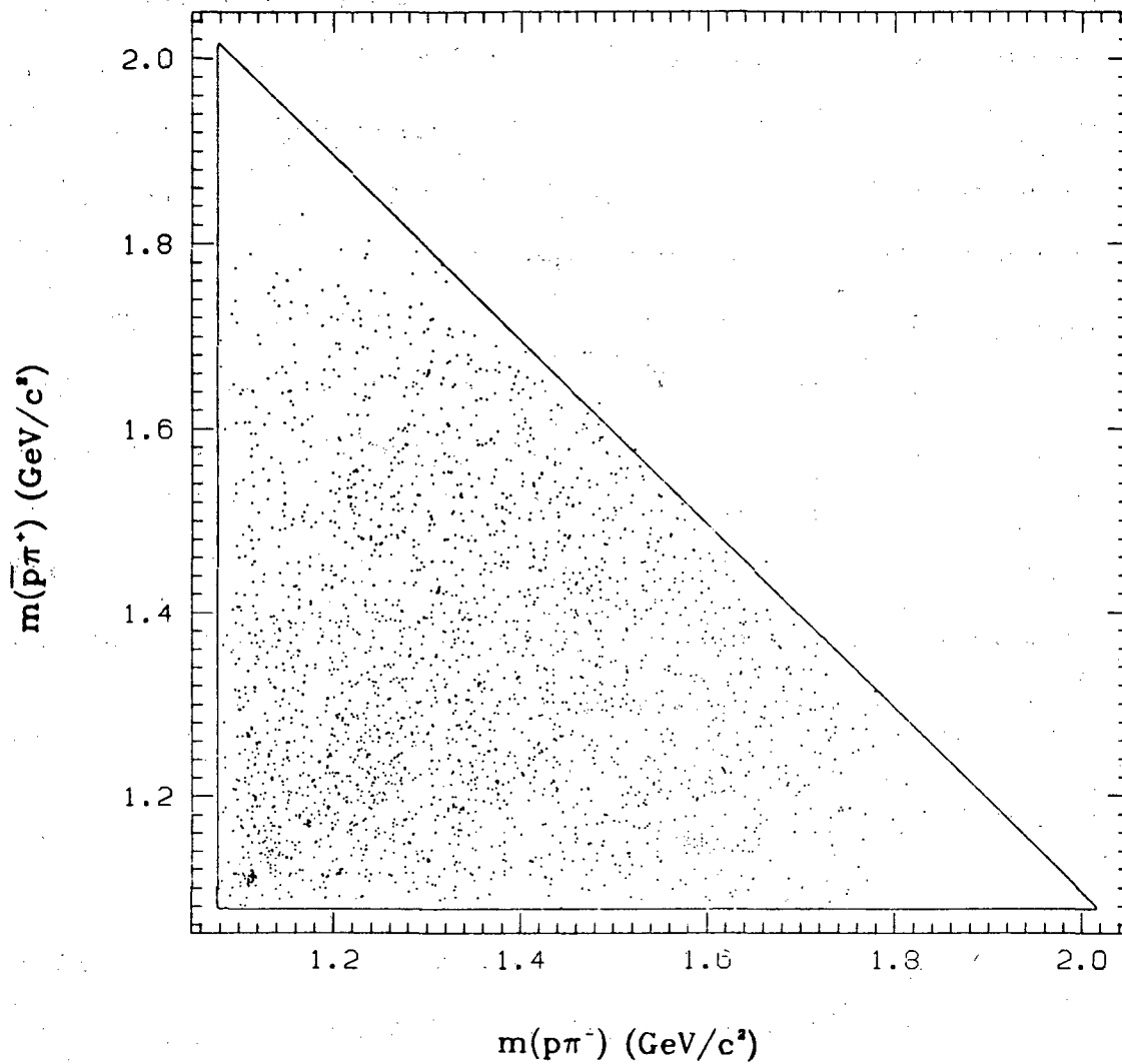
Figure 41: Goldhaber plot of m(p\pi^-) vs. m(\bar{p}\pi^+) .
