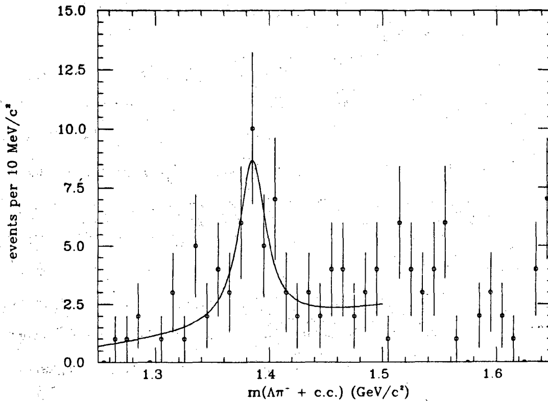
Figure 55: \Lambda\pi^- + \text{c.c.} mass opposite \Sigma recoil. Solid line is fit described in text.
