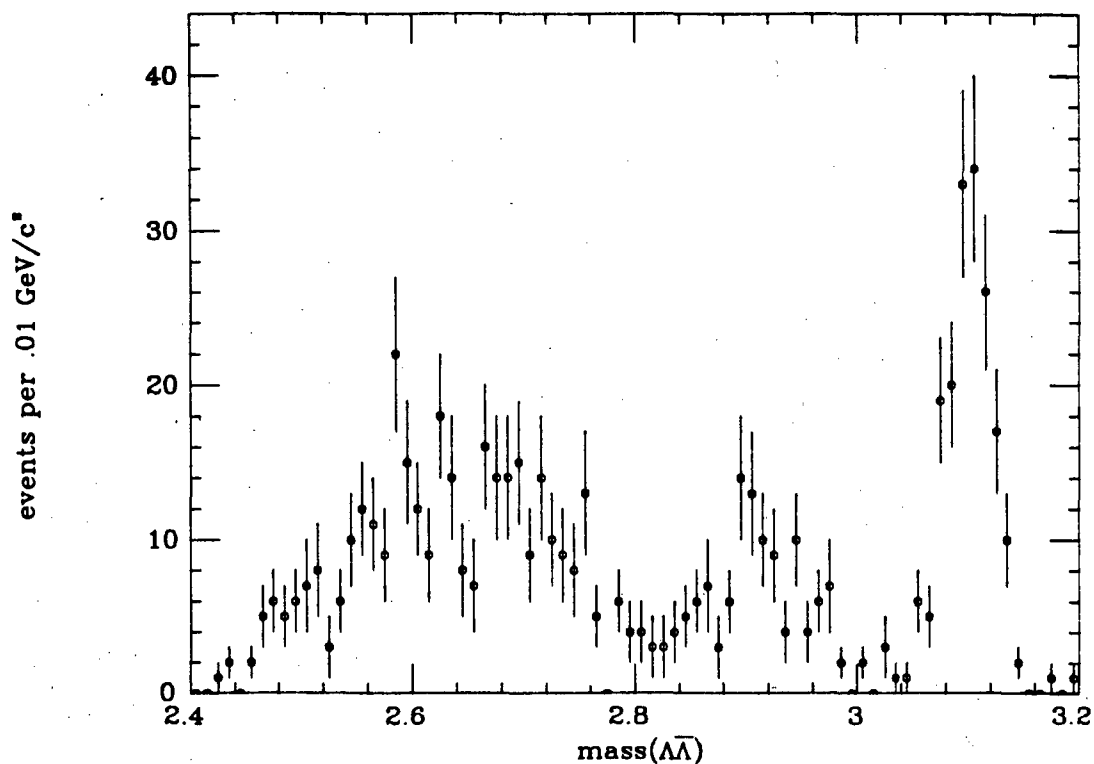
Figure 66: m(\Lambda\bar{\Lambda}) for all events.
