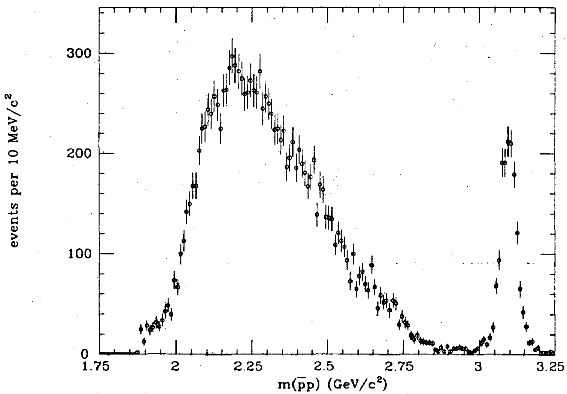
Figure 20: \bar{p}p mass for all pairs.
