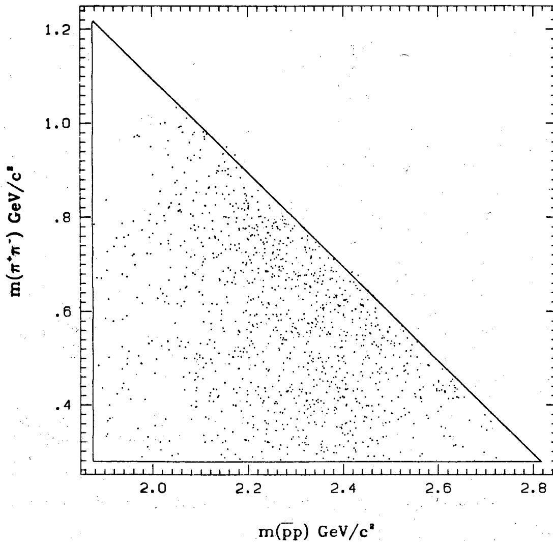
Figure 45: Goldhaber plot of m(\bar{p}p) vs. m(\pi^+\pi^-) . \Lambda\bar{\Lambda} and \Delta^{++}\bar{\Delta}^{--} subtracted.
