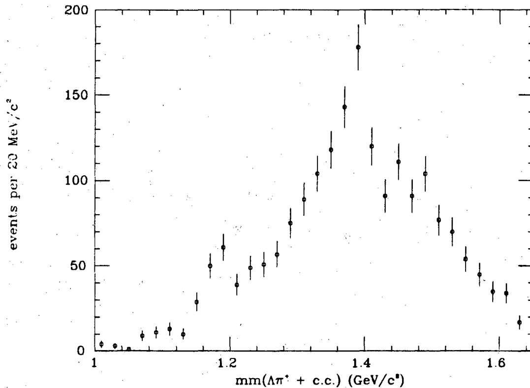
Figure 56: Missing mass opposite \Lambda\pi^+ + c.c. events.
