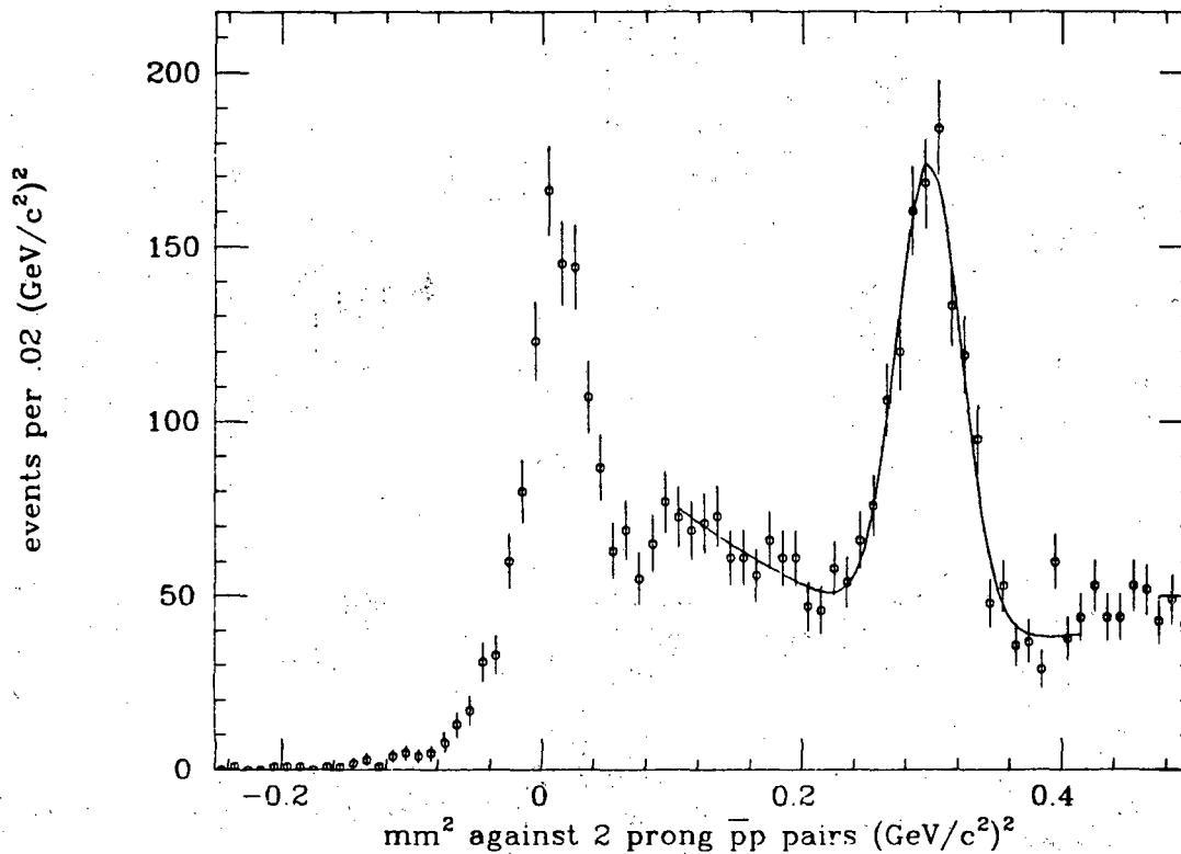
Figure 34: mm^2 against two prong \bar{p}p pairs at \psi .
