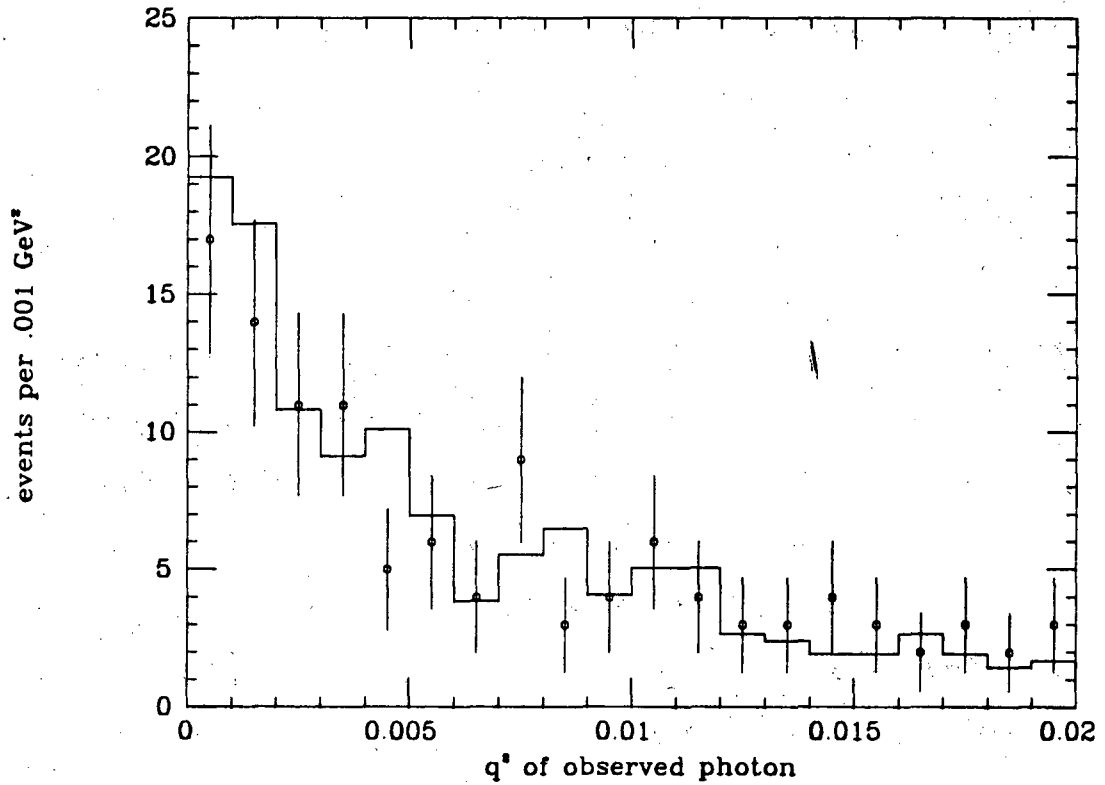
Figure 48: q^2 of observed photon.
