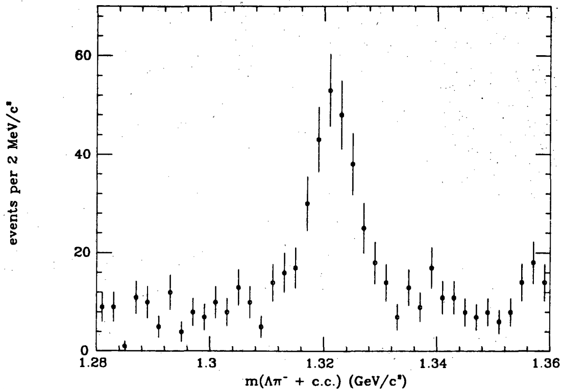
Figure 58: m(\Lambda\pi^- + \text{c.c.}) .
