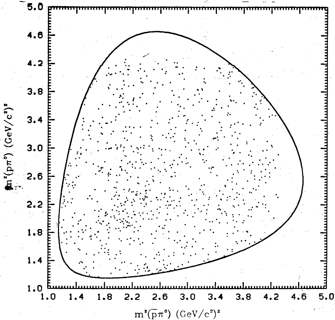
Figure 32: Dalitz plot for \psi \rightarrow \bar{p}p\pi^0 .
