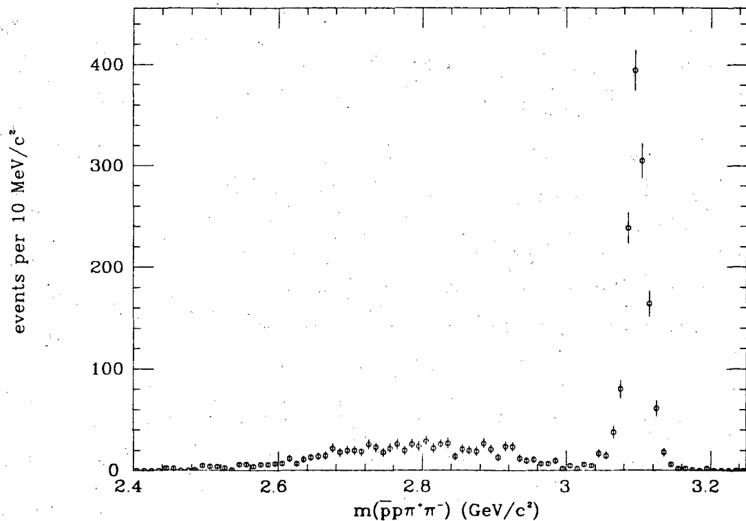
Figure 40: Mass plot for 4 prong \bar{p}p\pi^+\pi^- events.
