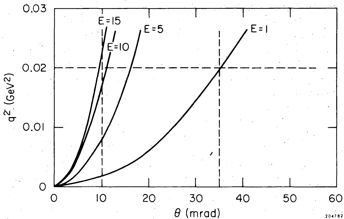
FIG. 1--Graphs of the electron momentum transfer |q^2| versus the lab scattering angle in mrad for various final electron energies.
