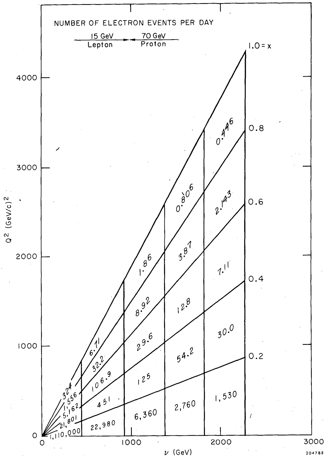
FIG. 3--Inelastic lepton scattering event rate using
