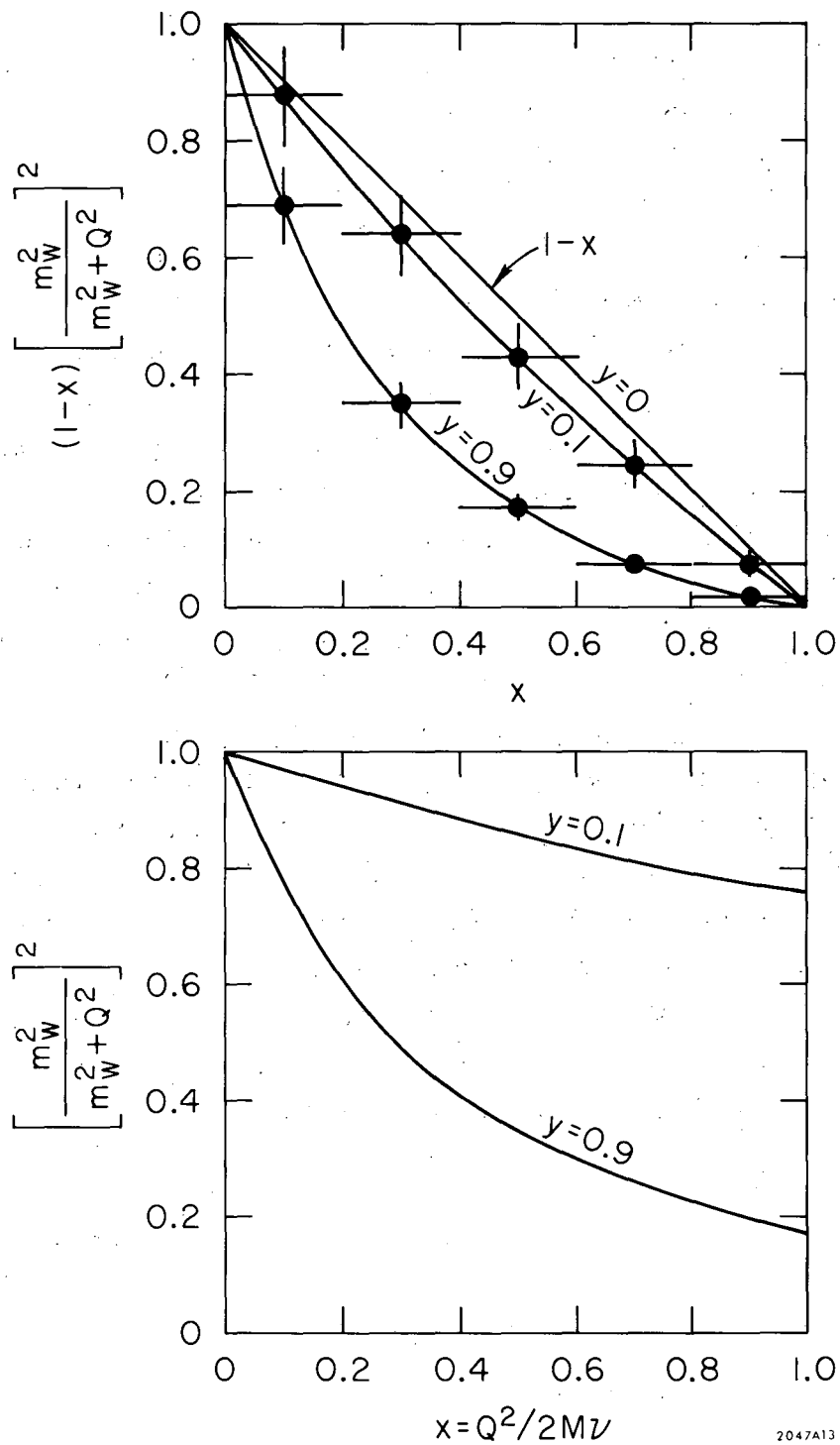
FIG. 6--How scaling for neutrino events would be broken by the existence of 53 GeV intermediate vector boson. Error bars correspond to a 10 day run. The variable x = Q^2/2M\nu ; y = \nu/\nu_{\max} .
