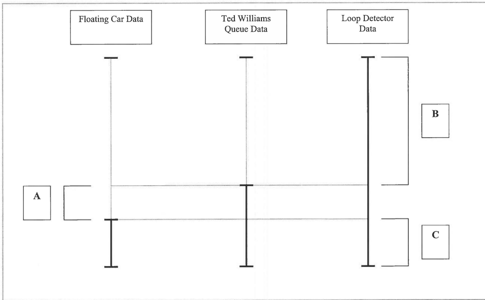
FIGURE 1: DATA STRUCTURE
