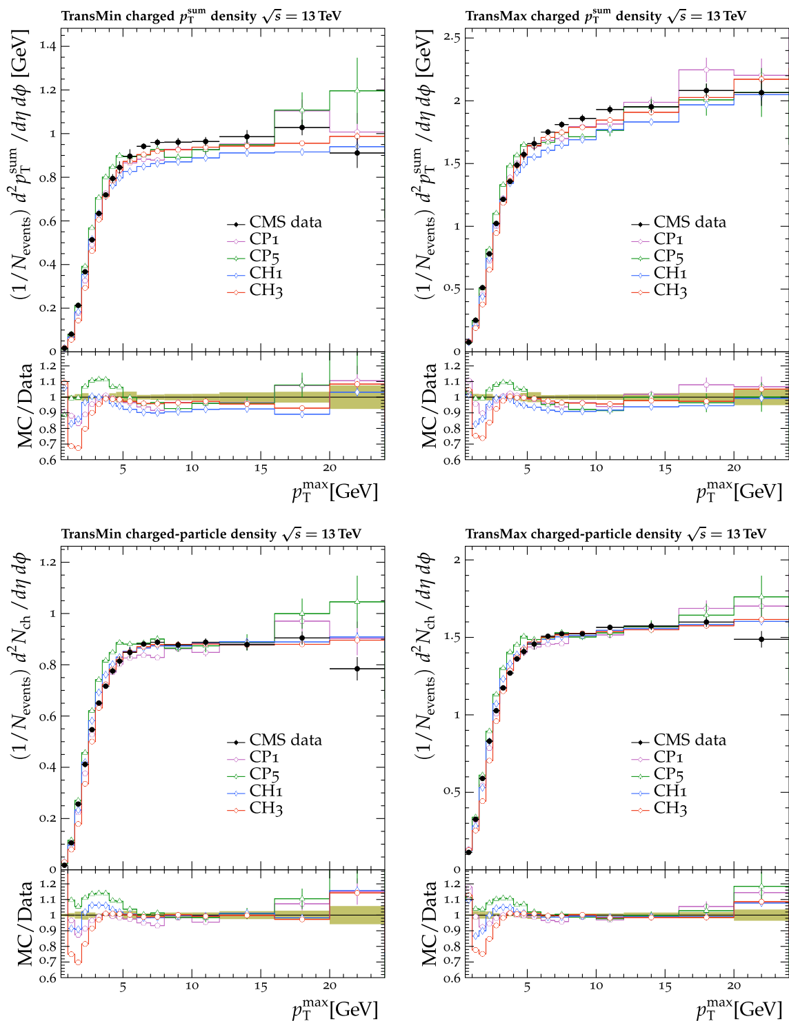
Fig. 7 The p_T^{\text{sum}} (upper) and N_{\text{ch}} (lower) density distributions in the transMin (left) and transMax (right) regions, as a function of the p_T of the leading track, p_T^{\max} [24]. CMS MB data are compared with the predictions from HERWIG 7, with the CH1 and CH3 tunes, and from
