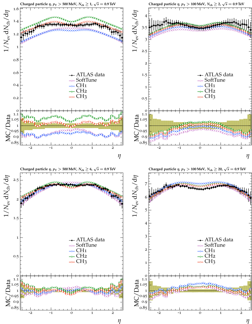
Fig. 20 Normalized plots [17] for the pseudorapidity of charged particles for N_{\text{ch}} \geq 1 (upper left), and N_{\text{ch}} \geq 6 (lower left), for charged particles with p_{\text{T}} > 500 MeV. The figure on the upper right shows a similar distribution for N_{\text{ch}} \geq 2 , and the lower right for N_{\text{ch}} \geq 20 , where the charged particles have p_{\text{T}} > 100 MeV. ATLAS MB data are compared with the predictions from HERWIG 7, with the SoftTune and CH tunes. The coloured band in the ratio plot represents the total experimental uncertainty in the data. The vertical bars on the points represent the statistical uncertainties
