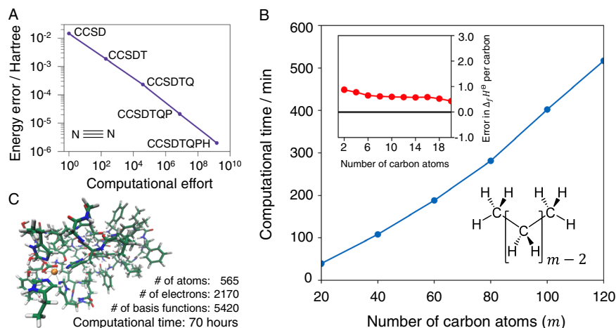
Fig. 3 | Computational complexity of classical heuristics for molecular systems.
