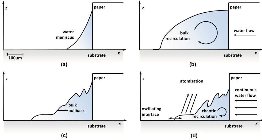
FIG. 2. (Color online) (a) At rest and prior to SAW actuation, a liquid meniscus formed between the wetted paper and the LN substrate. (b) Application of the SAW results in the pullout of a liquid bulk with height and length scales several times the liquid wavelength \lambda_l . (c) After \sim 50 – 500 ms, the leading edge of the liquid bulk was observed to retreat, (d) leaving behind a thin film region from which atomization occurred. The film and chaotic bulk liquid regions interacted dynamically, with the film moving horizontally and occasionally being obscured completely by the bulk region.
