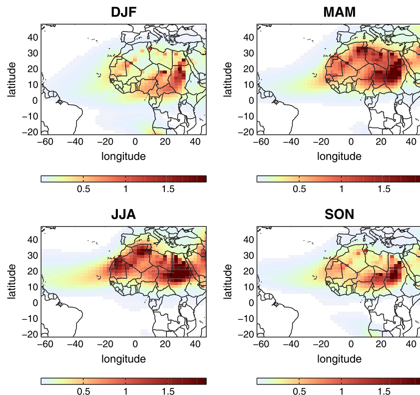
Figure 6. One hundred fifty year seasonal averages of CAM5 total dust burden ( \text{g}/\text{m}^2 ) for December-January-February (DJF), March-April-May (MAM), June-July-August (JJA), and September-October-November (SON).
