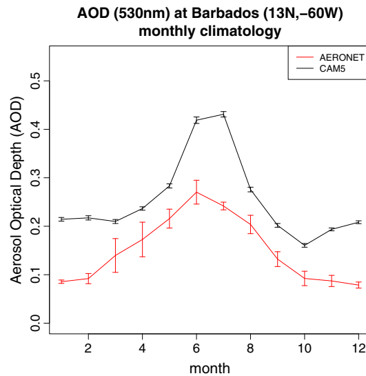
Figure 3. Mean monthly climatology of 530 nm aerosol optical depth (AOD) near Barbados (13°N, -60°W) from AERONET (red) and CAM5 (black). The AERONET data are available from 2007 to the present, and the CAM5 simulation is 150 years. Vertical bars represent ± 1 standard error for each month.
