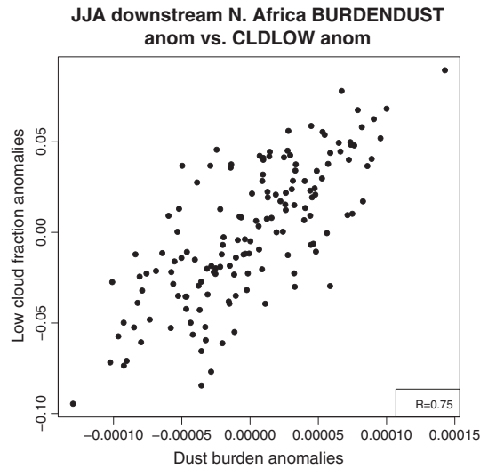
Figure 15. Scatterplot of boreal summer CAM5 average dust burden anomalies (abscissa; kg/m 2 ) and lower tropospheric cloud fraction anomalies (ordinate; unitless), area averaged over the modest-to-strong correlation region shown in Figure 14.
