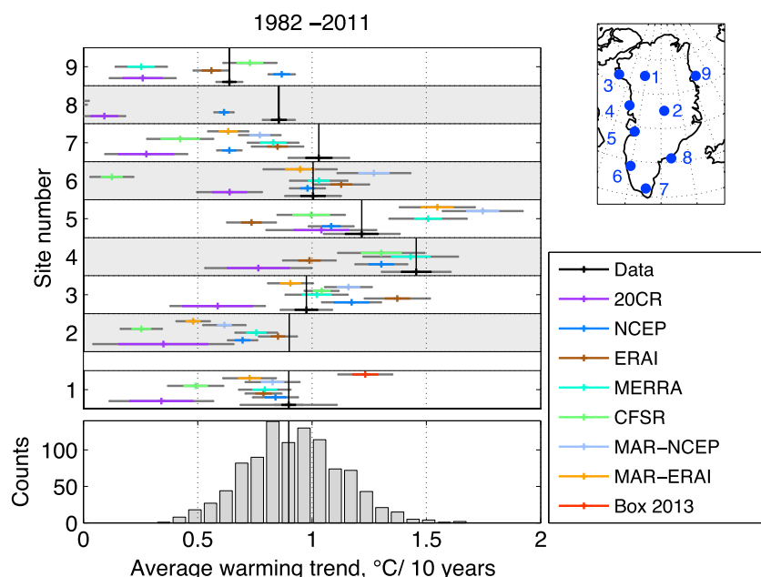
Figure 5. (bottom) Histogram of the calculated warming rate at NEEM (1) for the period 1982–2011. We find a warming of 0.91 \pm 0.21^\circ\text{C}/\text{decade} . (top) Warming rate from weather station data [Cappelen, 2014] (3, Pituffik; 4, Upernavik; 5, Ilulissat; 6, Nuuk; 7, Mittarfik; 8, Tasiilaq; and 9, Danmarkshavn) and Summit (2) [McGrath et al., 2013] are shown in black, and reanalysis outputs at the corresponding grid point. The trend at NEEM is similar to that of Summit and other Greenland coastal sites (3, 6, 7, and 8).
