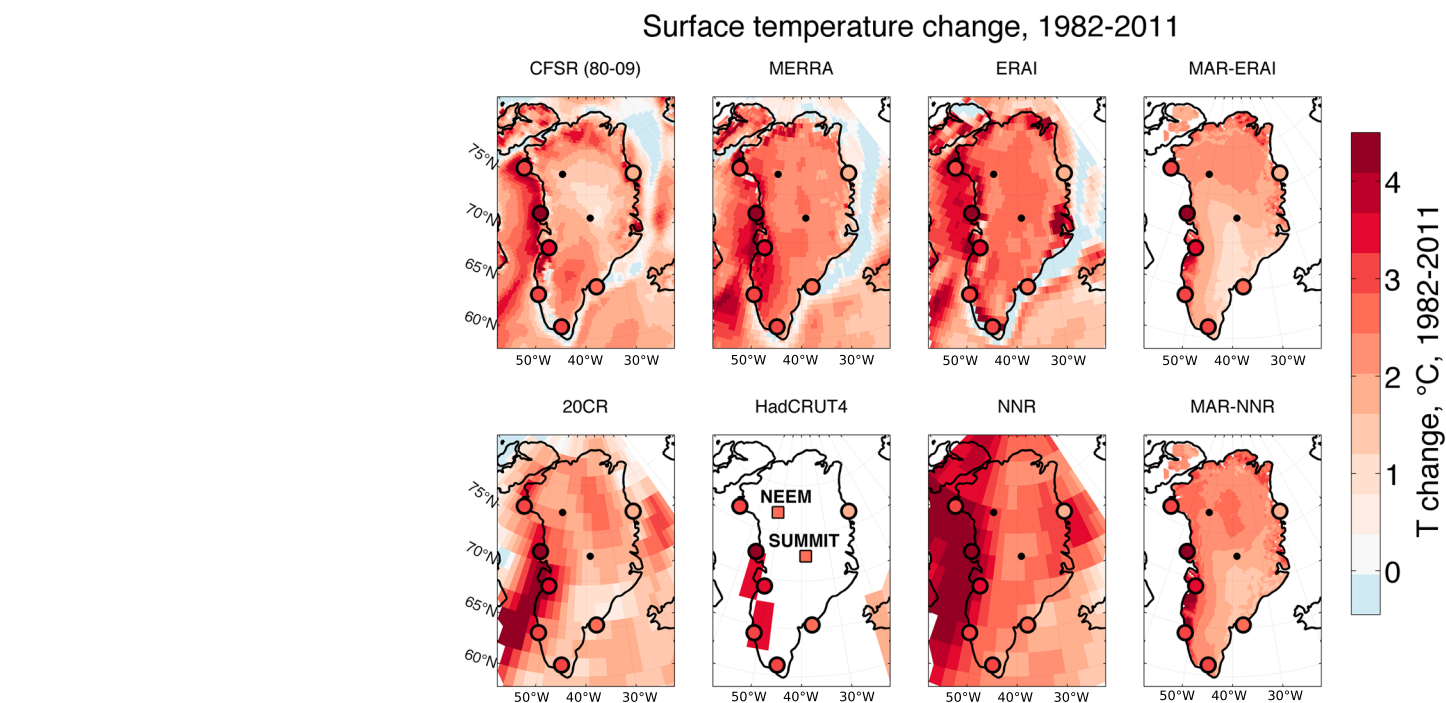
Figure 1. Thirty-year (1982–2011) surface temperature change from various reanalyses: NCEP-CFSR [Saha et al. , 2010], NASA-MERRA [Rienecker et al. , 2011], ERA-interim [Dee et al. , 2011], NCEP-20CR-v2c [Compo et al. , 2011], NCEP-NCAR reanalysis (NNR) [Kalnay et al. , 1996; Kistler et al. , 2001], as well as the outputs of the regional model MAR forced by either ERA-Interim or NNR [Fettweis et al. , 2013], and the surface temperature reconstruction from HadCRUT4 [Morice et al. , 2012]. The circles are trends calculated from all available weather stations having continuous measurements over the time period 1982–2011 [Cappelen, 2014]. The squares show the 30 year warming trend at NEEM (this work) and at Summit [McGrath et al. , 2013], the latter being based on the combination of firn temperatures and weather station data.
