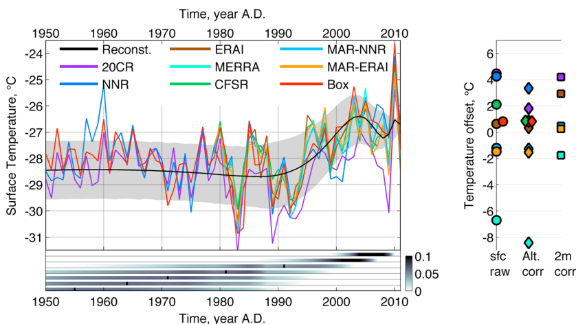
Figure 3. (left) Surface temperature reconstruction, from this inversion of borehole data and from a suite of atmospheric reanalyses: NCEP-20CR [Compo et al., 2011], NCEP-NCAR [Kalnay et al., 1996; Kistler et al., 2001], ERA-interim [Dee et al., 2011], NASA-MERRA [Rienecker et al., 2011], and NCEP-CFSR [Saha et al., 2010], as well as the outputs of the regional model MAR forced by either NCEP-NCAR or ERA-Interim [Fettweis et al., 2013] and an interpolation of weather station data from Box [2013]. (right) A constant temperature offset was used on each data set to match the absolute temperature (1982–2011 mean) measured in the NEEM borehole. The circles depict the raw offset between modeled surface temperature and borehole temperature, the diamonds show the offset after correcting the surface elevation bias (Alt. Corr), and the squares show the elevation-corrected bias in 2 m (3 m for MAR) temperature. The bottom bars show the age distributions of our reconstruction at several points in time. Before 1980, the reconstructed temperature is the average of many decades, which makes the curve look flat.
