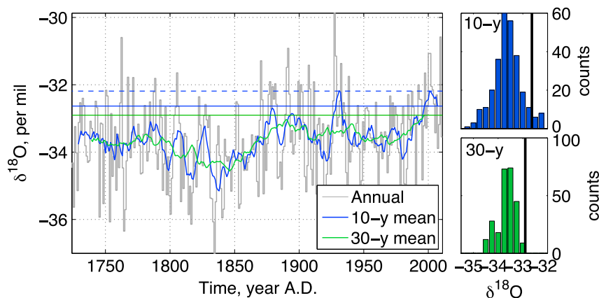
Figure 4. \delta^{18}\text{O} in a composite of four shallow ice cores from NEEM [Masson-Delmotte et al., 2015]. Annual mean (grey), 10 year running mean (blue), and 30 year running mean (green). The blue and green horizontal bars show the last 10 year mean and the last 30 year mean. Histograms on the right show the distribution to 10 (blue) and 30 year (green) temperature anomalies, and the most recent interval with a black bar. The recent warmest decade (1996–2005, dashed blue line) was superseded once in the last 287 years and is due to the large positive anomaly in 1928. The last 30 years are the warmest in the past 287 years.
