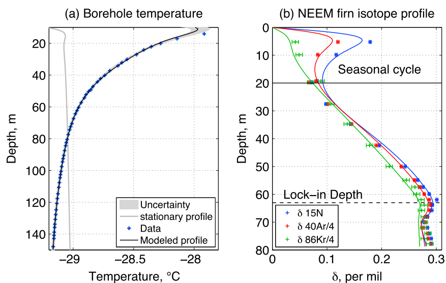
Figure 2. (a) Borehole temperature profile (+), with modeled fit to the data. A stationary temperature profile is shown in grey (run for 20 ka at -29.2^{\circ}\text{C} ). The temperature increase toward the surface indicates a warming trend. (b) Inert gas isotope data (+) and model fit (lines) from our best solution. The top 20 m signal shows the response to the seasonal cycle. Krypton isotopes (green) are the least sensitive to temperature and a good proxy for gravitational fractionation. The deviation between nitrogen isotopes (blue) and krypton isotopes (green) is the thermal signal. The lock-in depth is the horizon where advection dominates gas transport, and gravitational fractionation effectively stops.
